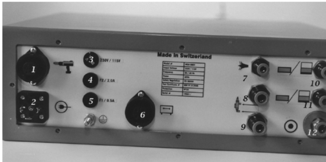
Illustration 14 Rear view of the 5800 Series unit
