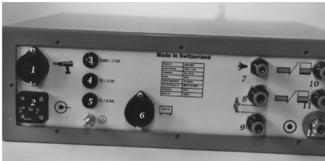
Illustration 12 Rear view of the 5800 Series unit
