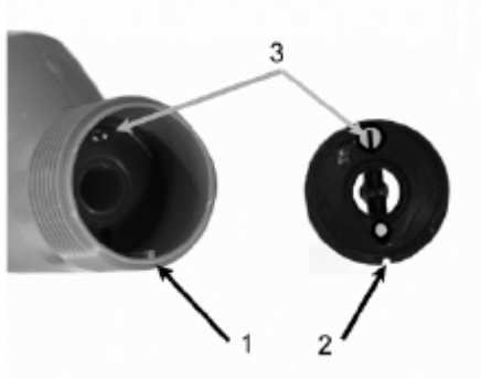
Illustration 14 Electrode holder position at gun reassembly
