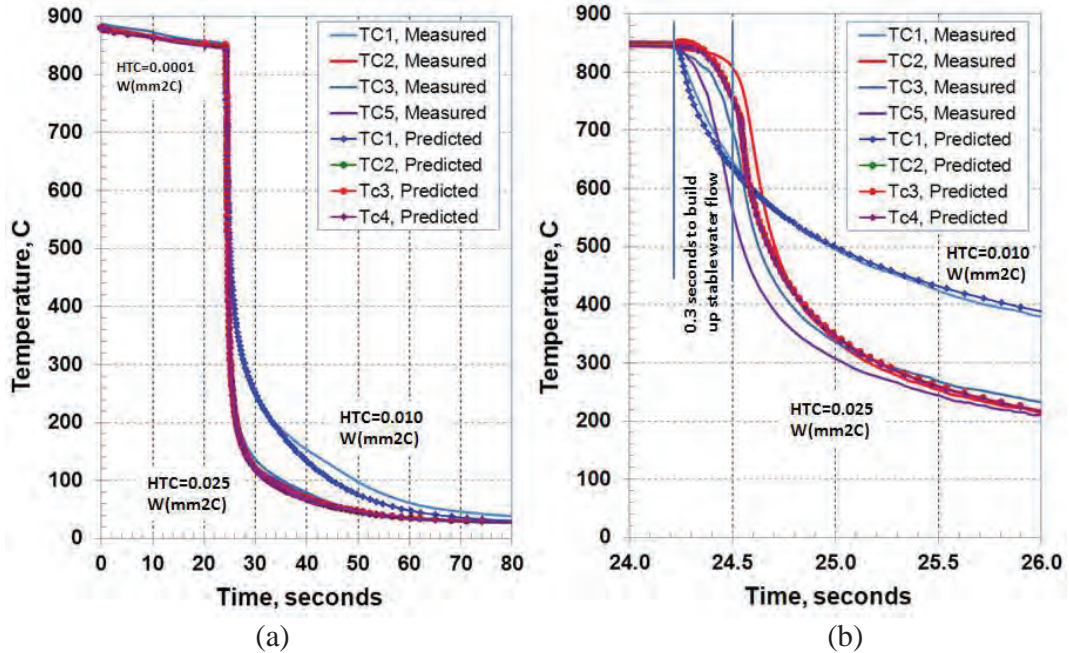
Figure 9 (a) Predicted and Measured Temperature vs. Time Results for Test #1, and (b) Magnified View of the Temperature vs. Time Predictions and Measurements for Test #1. Time for Achieving Full Water Flow is Identified.
