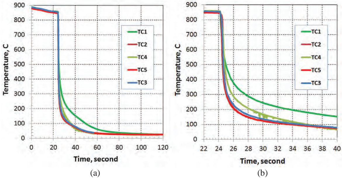
Figure 5 (a) Quenching Data for Test #1, (b) Magnified View of Initial Quenching Data for Test #1 .
