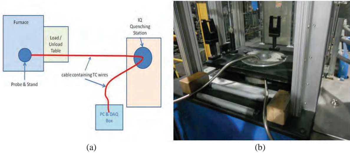
Figure 2 (a) Schematic of Intensive Quenching Test Setup, and (b) Cable Threaded Through the Intensive.
