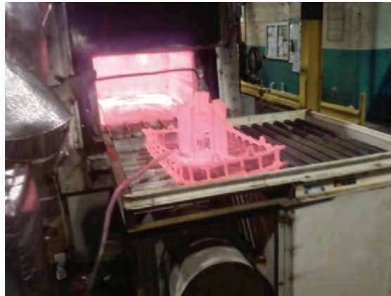
Figure 3 Hot Probe in Hot Stand After Removal from Furnace.
