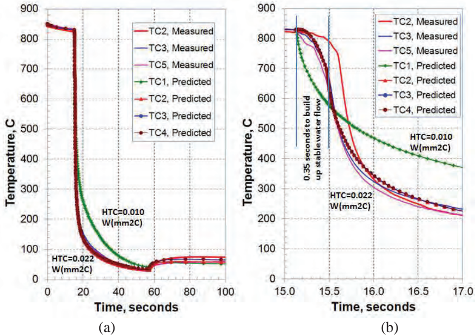
Figure 10 (a) Predicted and Measured Temperature vs. Time Results for Test #2, (b) Magnified View of Predicted and Measured Temperature vs. Time Results for Test #2 Showing Transition Period to Full Water Flow.
