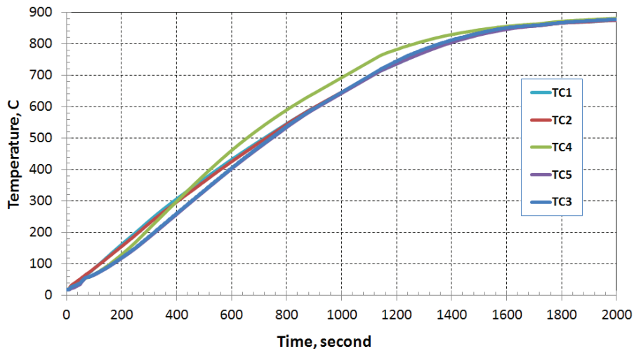
Figure 4 Heating Data for Test #1.
