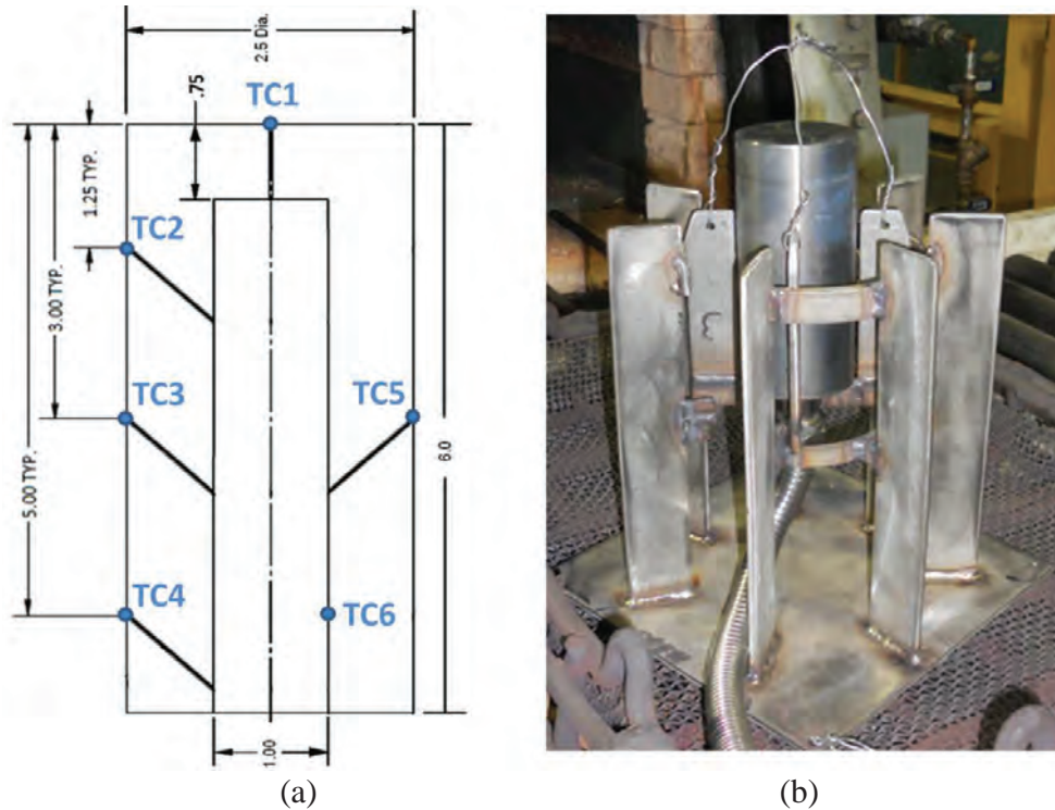
Figure 1 (a) Drawing of 304 SS Quench Probe Body Showing Thermocouple Locations, and (b) Probe Loaded onto Furnace Stand Prior to Loading into the Heated Furnace.
