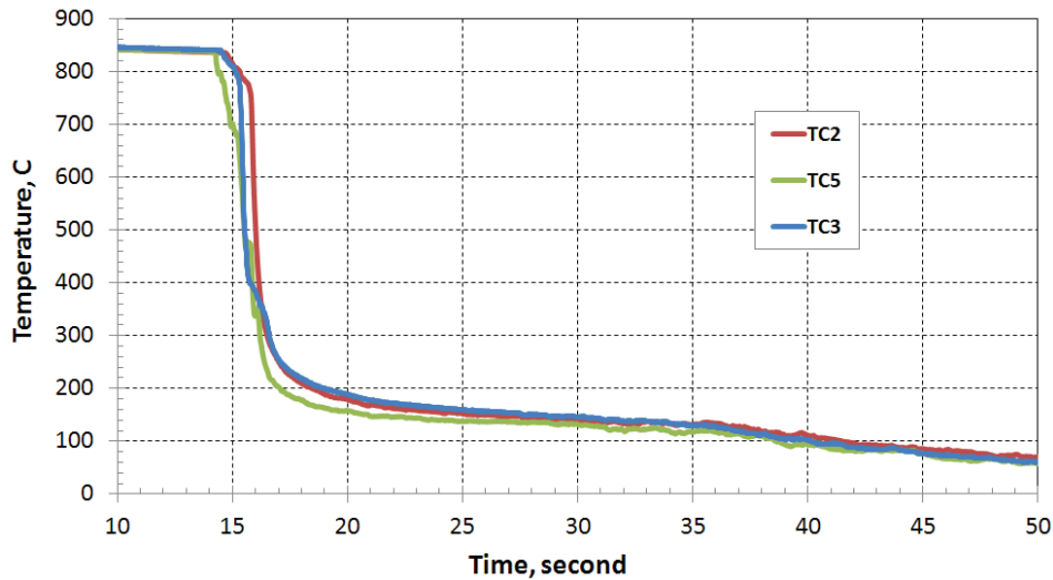
Figure 7 Data for Agitated Water Quench - Test #3.
