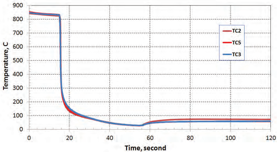
Figure 6 Quenching and Air Cooling Data for Test #2.
