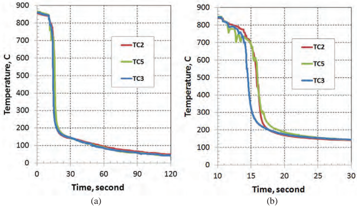
Figure 8 (a) Data for Quenching in Still Water - Test #4, and (b) Magnified View of Initial Data for Quenching in Still Water - Test #4.
