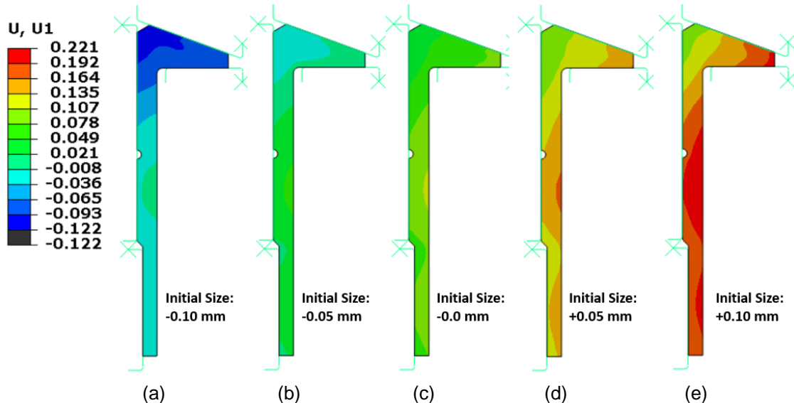
Figure 16 – Effect of initial gear size on predicted radial displacements using the press quench with 10 KN expander load and 850° C austenitizing temperature. a) -0.10 mm, b) -0.05 mm, c) 0.0 mm, d) +0.05 mm, and e) +0.10 mm.
