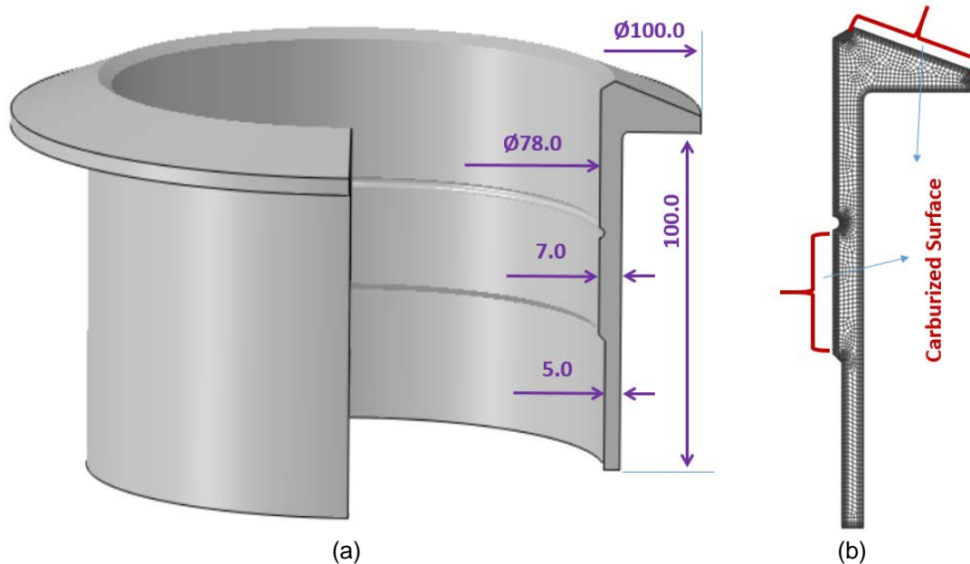
Figure 2 – Simplified thin-wall bevel gear. a) CAD model and dimensions, and b) Finite element mesh.
