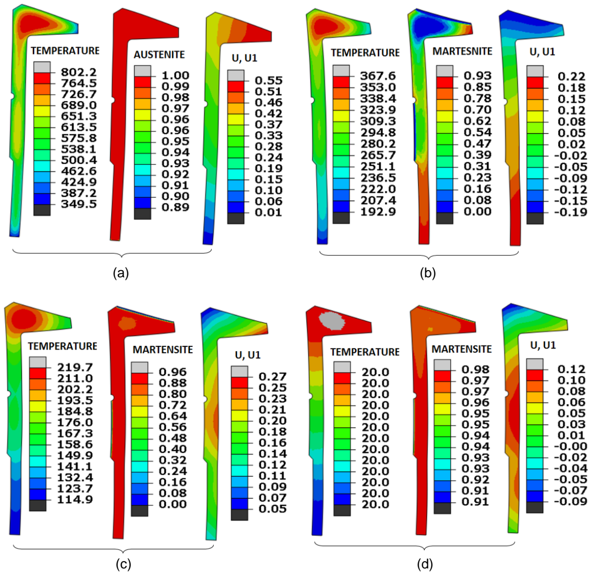
Figure 5 – Temperature, austenite/martensite and radial displacement distribution contours during quenching.
