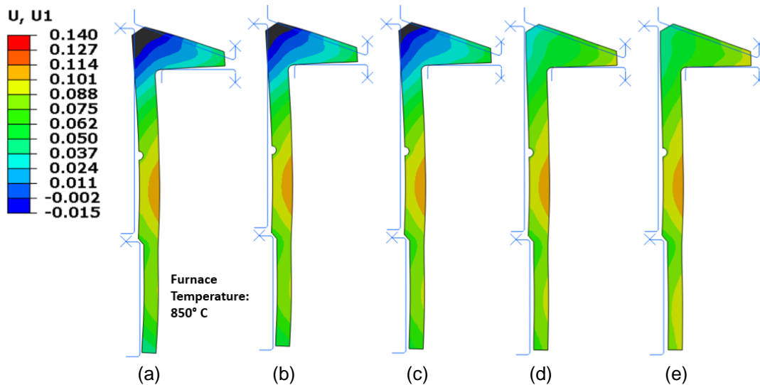
Figure 10 – Effect of expander load on predicted radial displacement using press quench with 850° C austenitizing temperature. a) 2.5 KN, b) 5.0 KN, c) 7.5 KN, d) 10.0 KN, and e) 15.0 KN.
