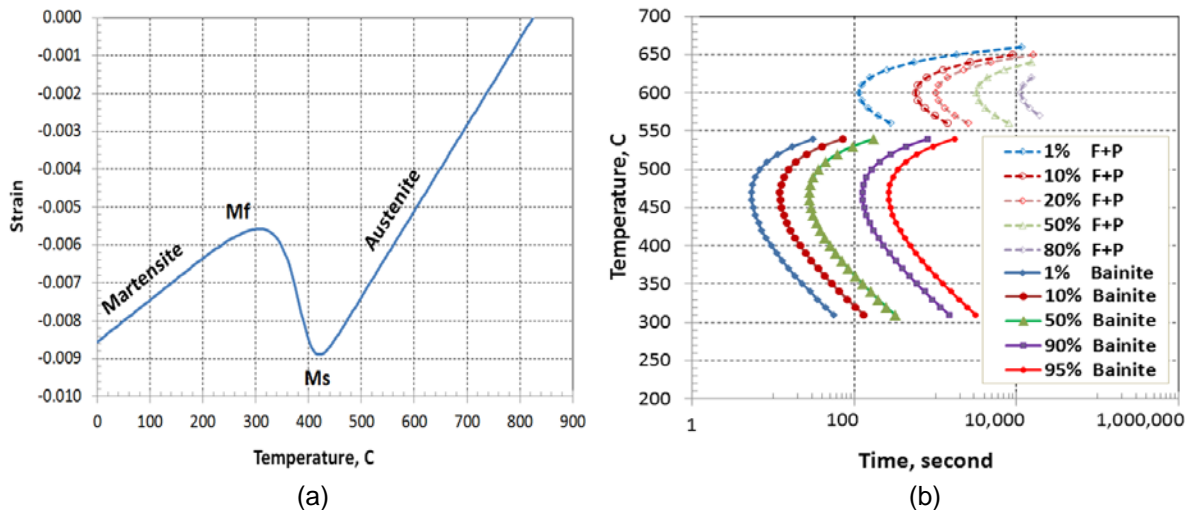
Figure 1 – a) Dilatometry strain curve with martensitic transformation, and b) TTT diagram of diffusive transformation for AISI 9310 steel.
