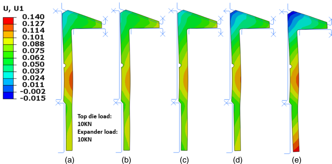
Figure 11 – Effect of austenitizing temperature on predicted radial displacement using press quench with a 10 KN load on top die and a 10 KN load on the expander. a) 810° C, b) 825° C, c) 850° C, d) 875° C, e) 900° C.
