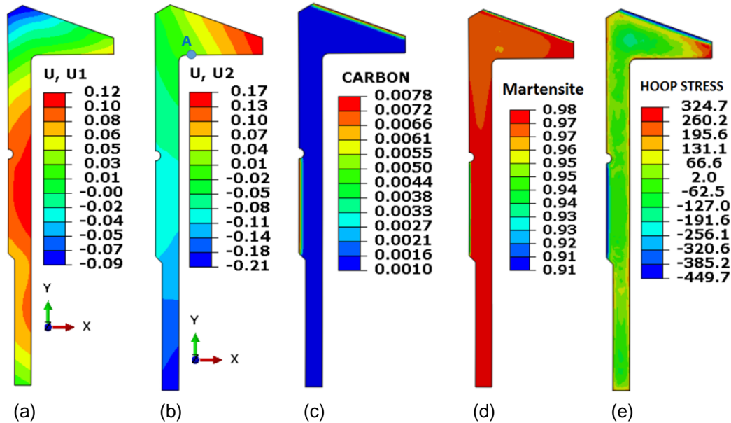
Figure 3 – Modeling results of immersion oil quench process. a) radial displacement, b) axial displacement, c) carbon fraction, d) martensite fraction, and e) circumferential residual stress.
