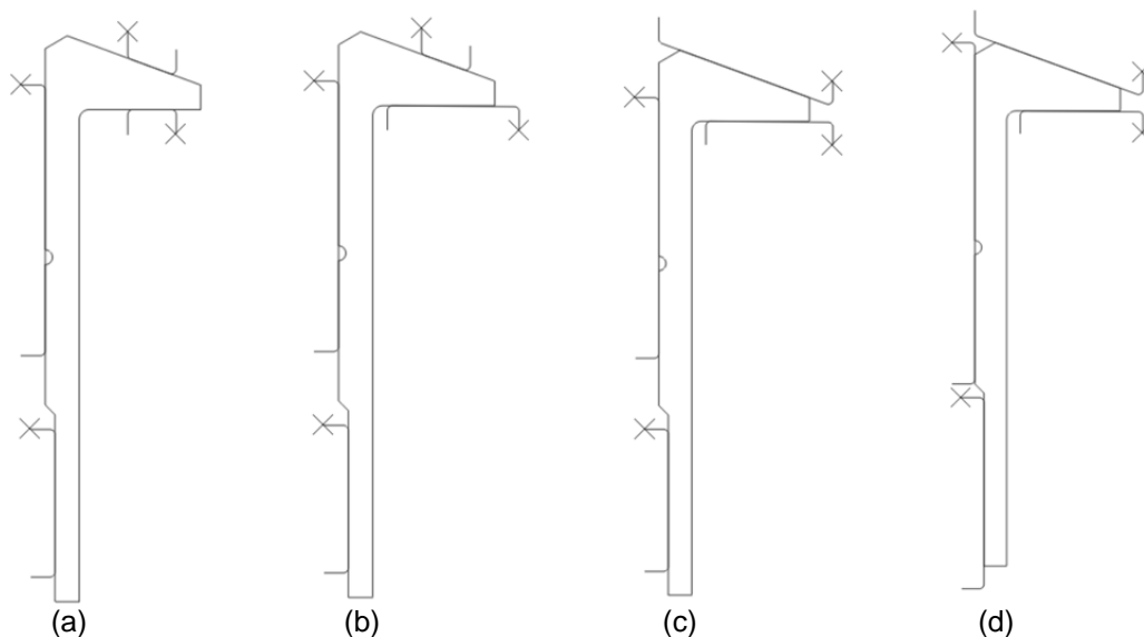
Figure 6 – Press/Plug quenching tooling design. a) tooling-1, b) tooling-2, c) tooling-3, and d) tooling-4.
