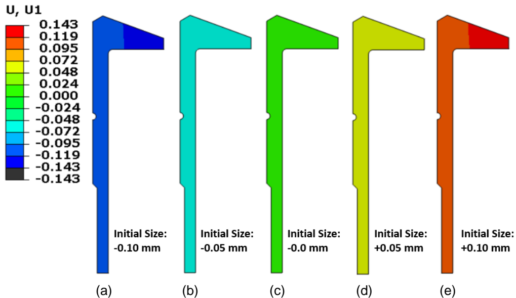
Figure 15 – Radial displacement contours (initial gear sizes) of the gear at room temperature prior to heating. a) -0.1 mm, b) -0.05 mm, c) 0.0 mm, d) +0.05 mm, and e) +0.1 mm.
