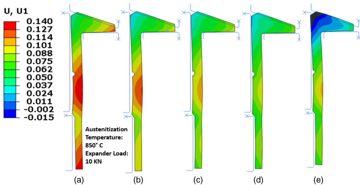
Figure 13 – Effect of quenching rate on predicted radial displacement using press quench with 850° C austenitizing temperature and 10 KN expander load. a) 50% HTC, b) 75% HTC, c) 100% HTC, d) 125% HTC, and e) 150% HTC.
