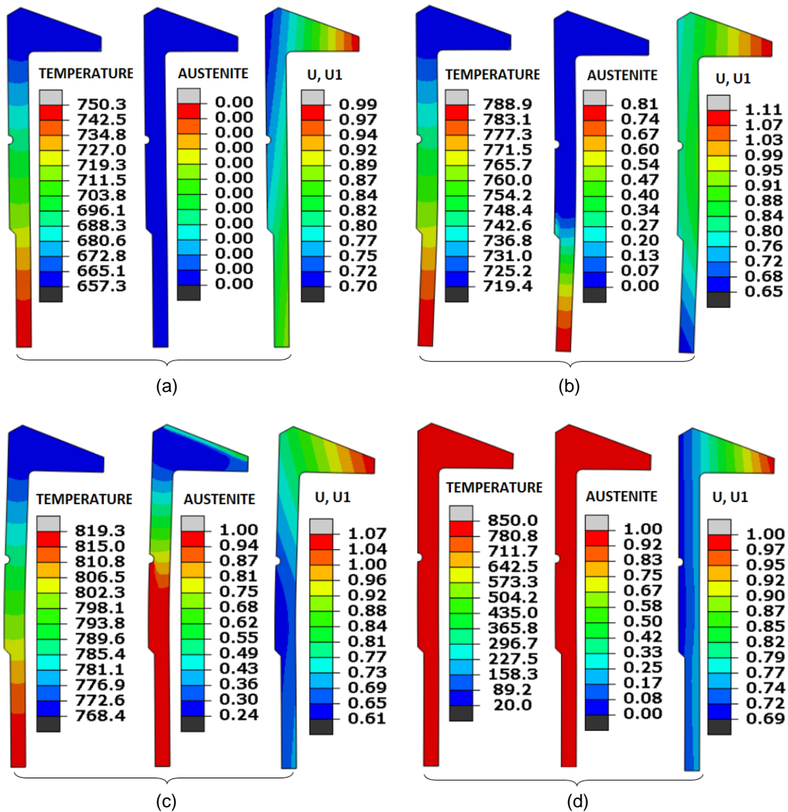
Figure 4 – Temperature, austenite and radial displacement distribution contours during heating process. a) at 422.6 s, b) at 515.5 s, c) at 627.0 s, and d) at the end of heating.
