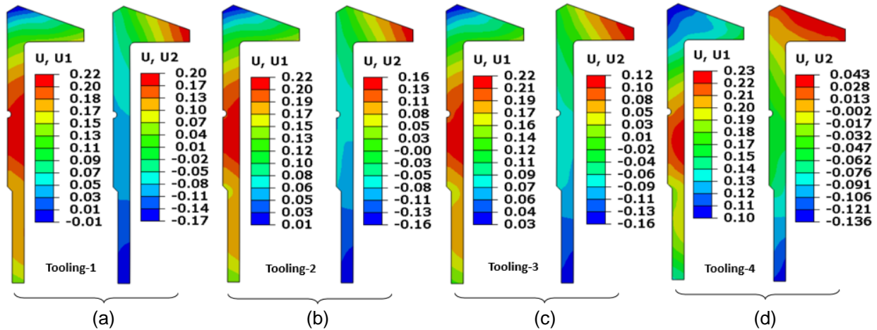
Figure 7 – Predicted radial and axial displacements from press quench model using the plug design with +0.0 mm plug size and 10 KN load applied on the top die. a) tooling-1, b) tooling-2, c) tooling-3, and d) tooling-4.
