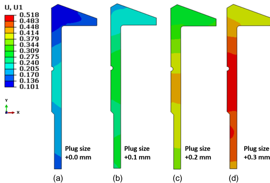
Figure 9 – Effect of plug size on predicted radial displacements with the tooling-4 design and 10 KN applied on the top die.
