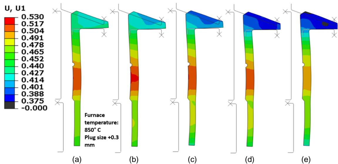
Figure 14 – Effect of quenching rate on predicted radial displacement using the plug quench with 850° C austenitizing temperature and plug +0.3 mm tooling design. a) 50% HTC, b) 75% HTC, c) 100% HTC, d) 125% HTC, and e) 150% HTC.
