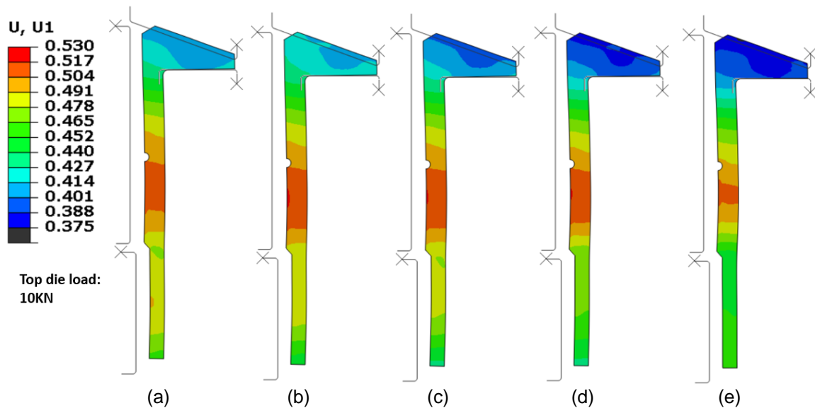
Figure 12 – Effect of austenitizing temperature on predicted radial displacement using press quench with 10 KN load on top die and plug +0.3 mm design. a) 810° C, b) 825° C, c) 850° C, d) 875° C, e) 900° C.
