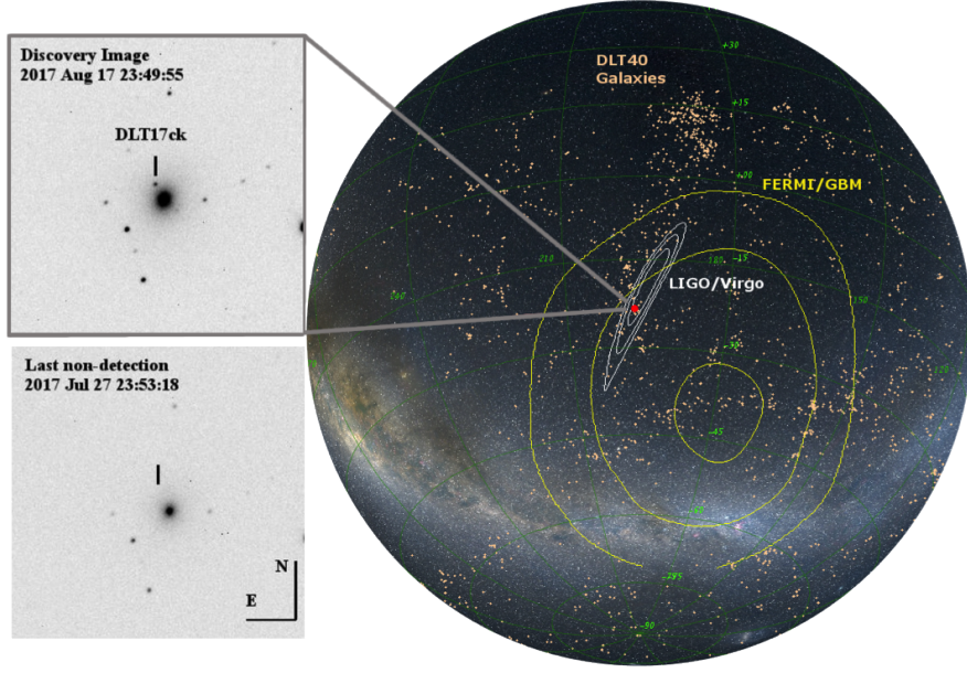
Figure 1: The right panel shows the localization of the GW170817 LVC event using all three gravitational-wave observatories (H1, L1, and V1; 31 \text{ deg}^2 ), over-imposed on the Fermi localization of GBM trigger GRB170817a. The DLT40 galaxy catalogue are marked in orange. The red point marks the location of DLT17ck and the host galaxy NGC 4993. The inset shows the discovery of DLT17ck in host galaxy NGC 4993 (top left) and the pre-discovery image from 20.5 days prior to merger (bottom left).
