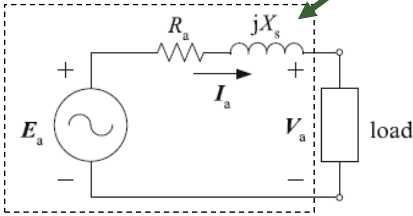
Generator Equivalent Circuit (per-phase)
