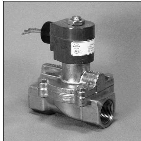
3/8", 1/2" and 3/4" NPT anti-water hammer solenoid valves in brass & nickel-plated brass body materials with stainless steel trim.
