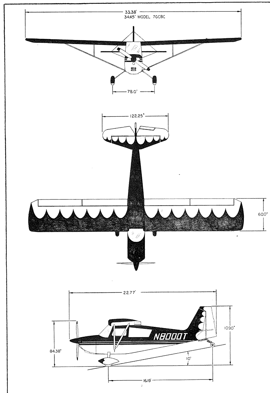
FIGURE 6-2 CITABRIA THREE-VIEW
