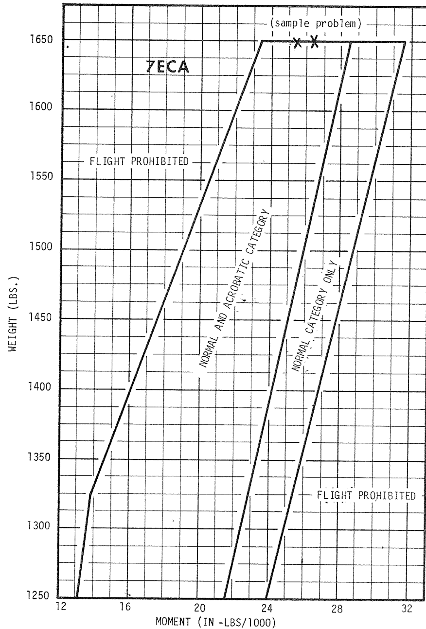
FIGURE 5-3 FLIGHT ENVELOPE - 7ECA ONLY
