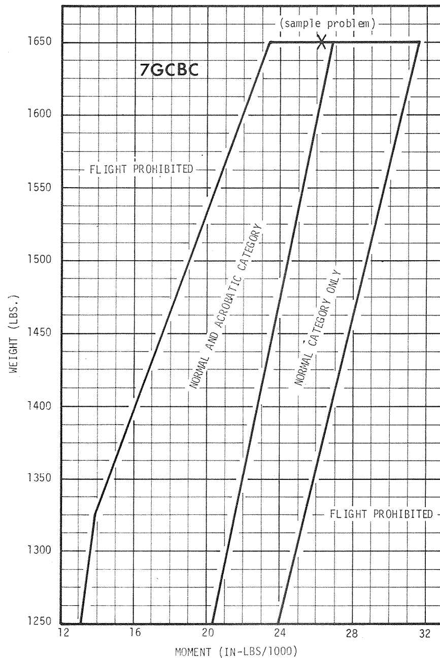
FIGURE 5-5 FLIGHT ENVELOPE - 7GCBC ONLY
