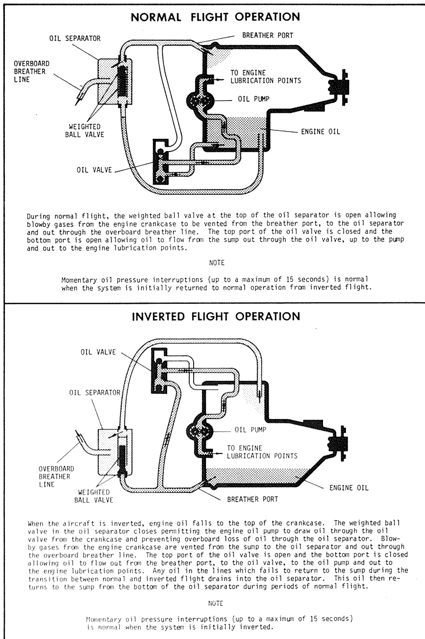
FIGURE 6-3 INVERTED ENGINE OIL SYSTEM (7KCAB ONLY)
