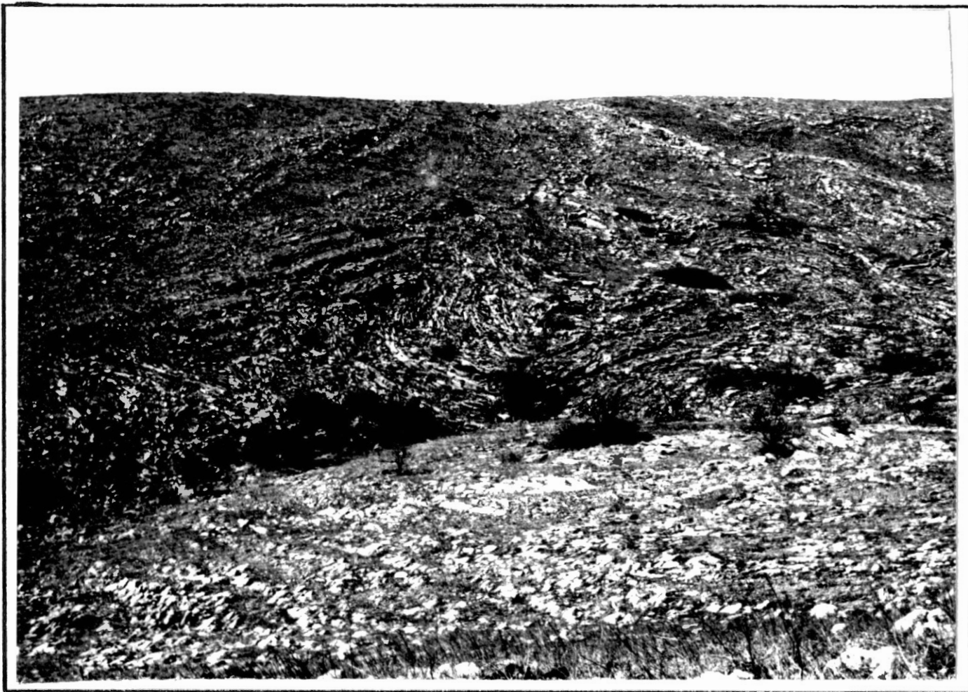
Figure 29. Disharmonic Character of Beds in the Disturbed Zone North of the Kiowa Syncline
