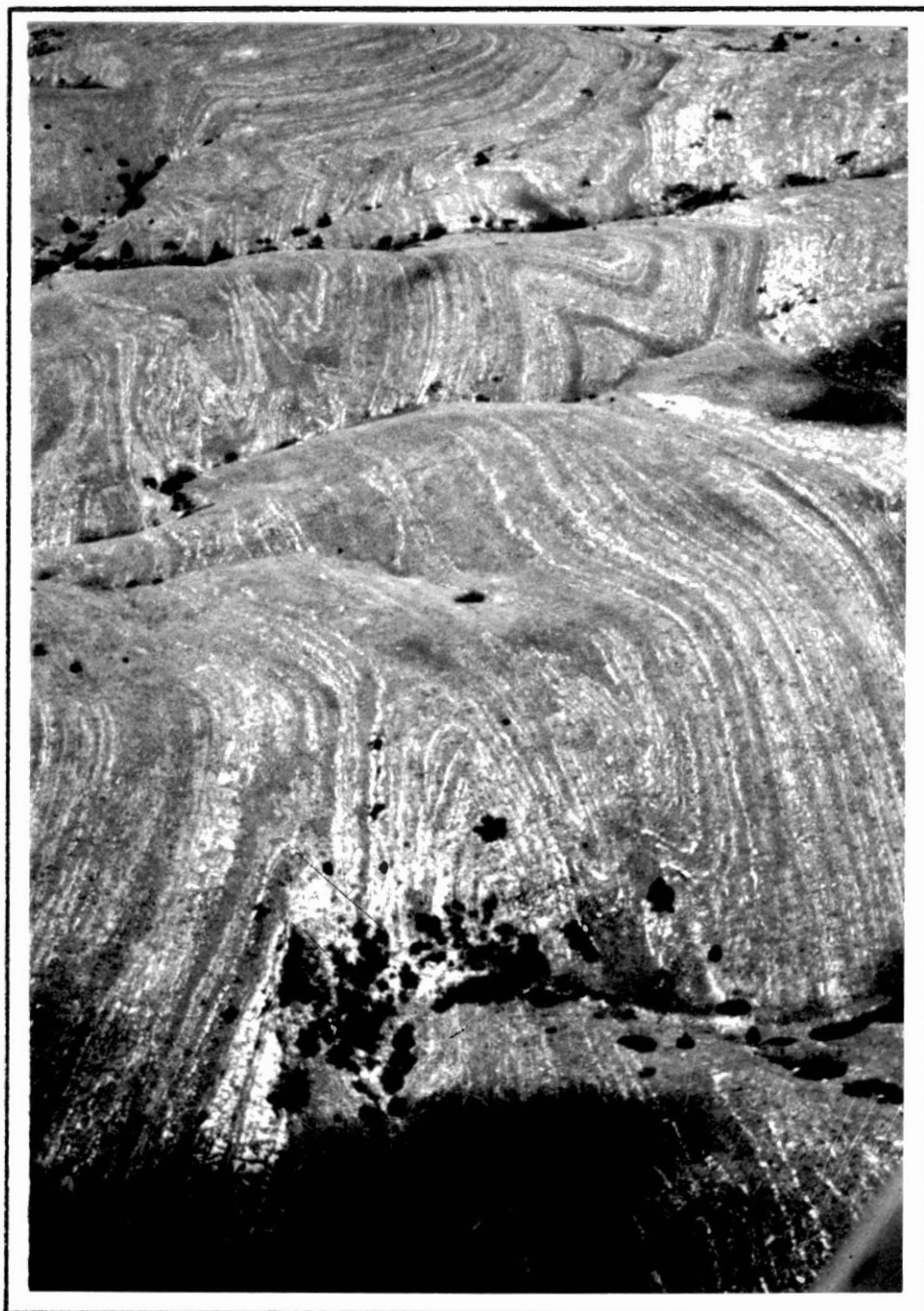
Figure 36. Minor Folding Associated With the Bat Cave Fault Within the Tully Disturbed Zone. Looking Northward Across the S\frac{1}{2} of Sec. 24 and the N\frac{1}{2} of Sec. 25. High Angle Reverse Fault in the Left (west) of Picture as it Dies out a Fold Pair to the East (air photo)
