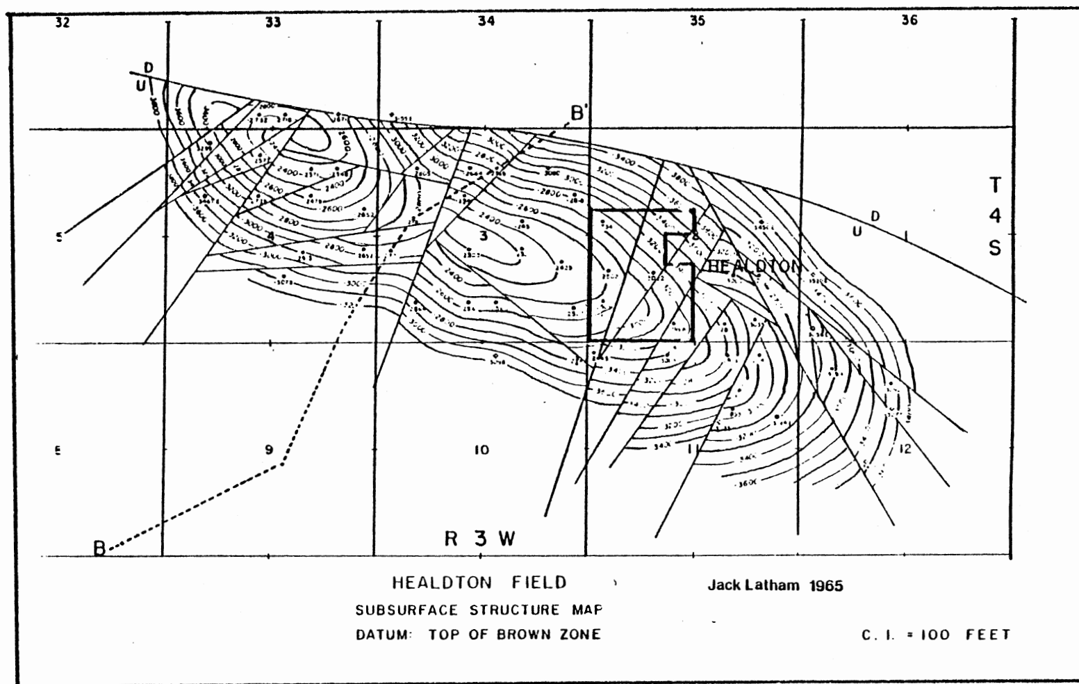
Figure 54. Subsurface Structure Map of the Healdton Field. Asymmetrical Anticline is Faulted Along the Northeast Limb
