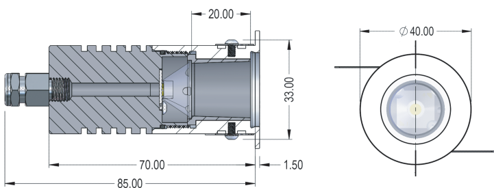
CUT-OUT - 32Ø
