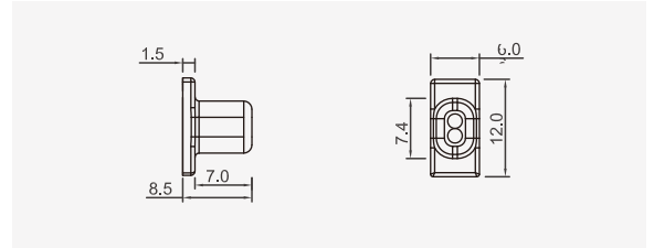
Integral plug
