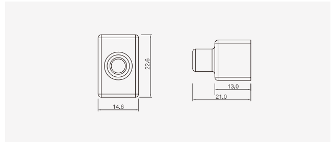
Integral plug
