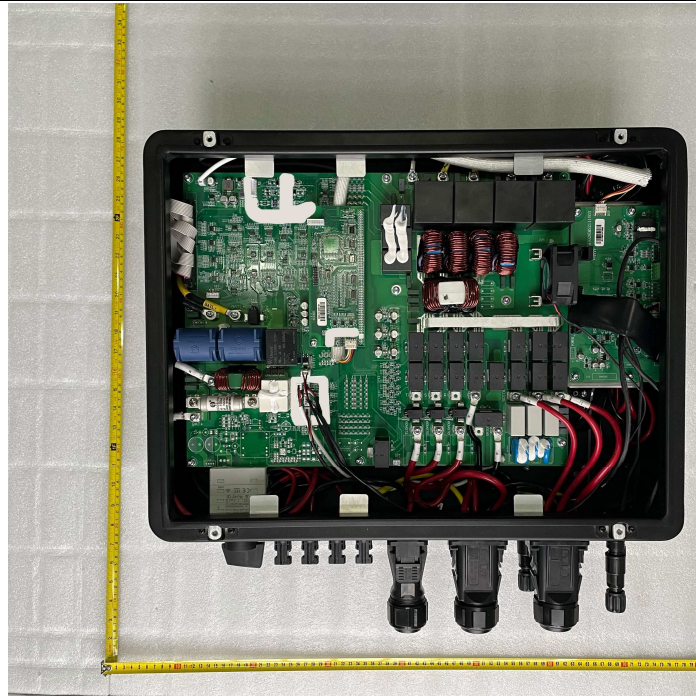
Internal view-
