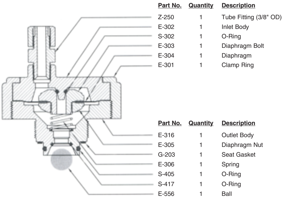
A-305 High/Low Pressure Ball Check Valve Assembly - 100 PPD (2000 GM/HR) Maximum
