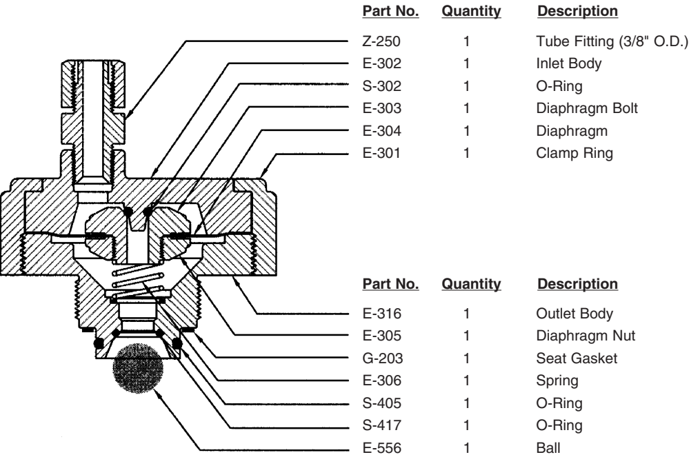
A-305 HIGH/LOW PRESSURE BALL CHECK VALVE ASSEMBLY 100 PPD (2000 GM/HR) MAXIMUM
