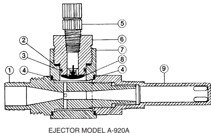
Ejector Assembly A-920A Check Valve Assembly E-225A Includes Ref No. 2, 3, 5, 6, 8 Max. Capacity: 100 lbs./24 hrs. (2000 g/hr)
