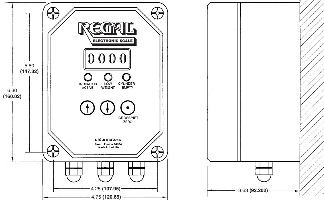
A) Single Cylinder (Model ECS401) Electronic Scale Monitor
