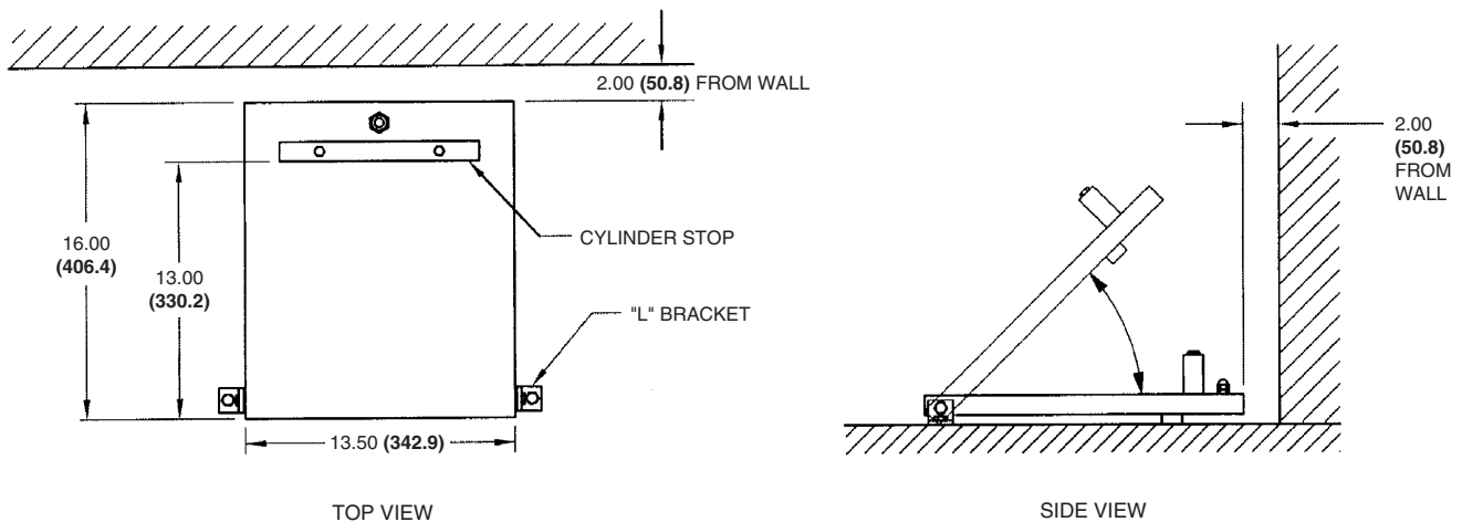
C) Scale Base Installation
