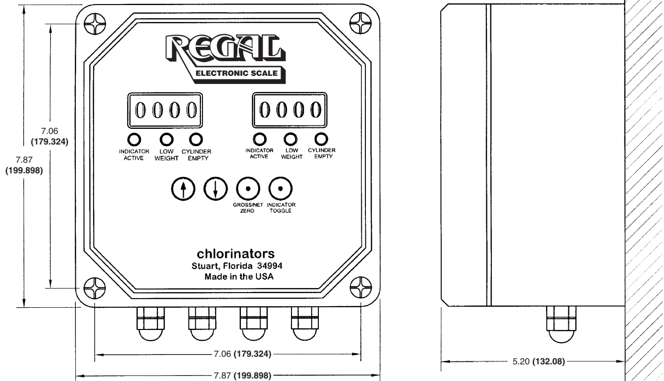
B) Dual Cylinder (Model ECS402) Electronic Scale Monitor
