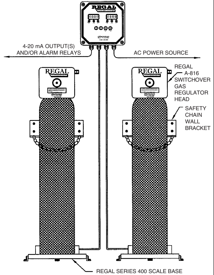
B) REGAL Model ECS402 Dual Cylinder Electronic Scale
