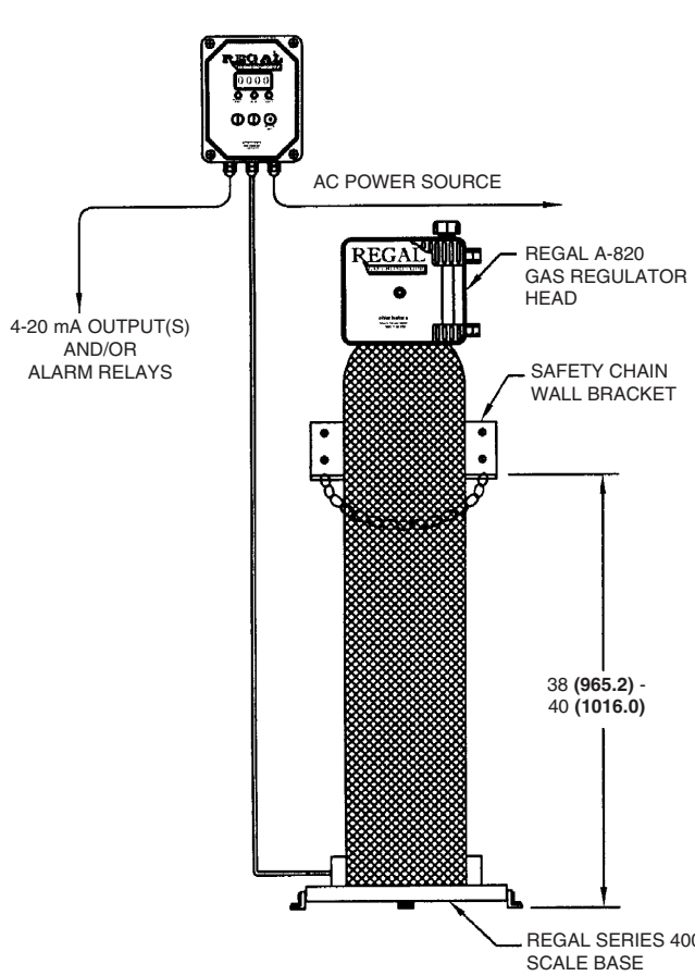
A) REGAL Model ECS401 Single Cylinder Electronic Scale
