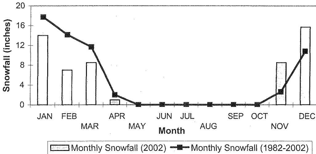
Figure 8: Lakeport 2 Climatological Sampling Station (Laconia, NH) Monthly Snowfall (1982-2002)
