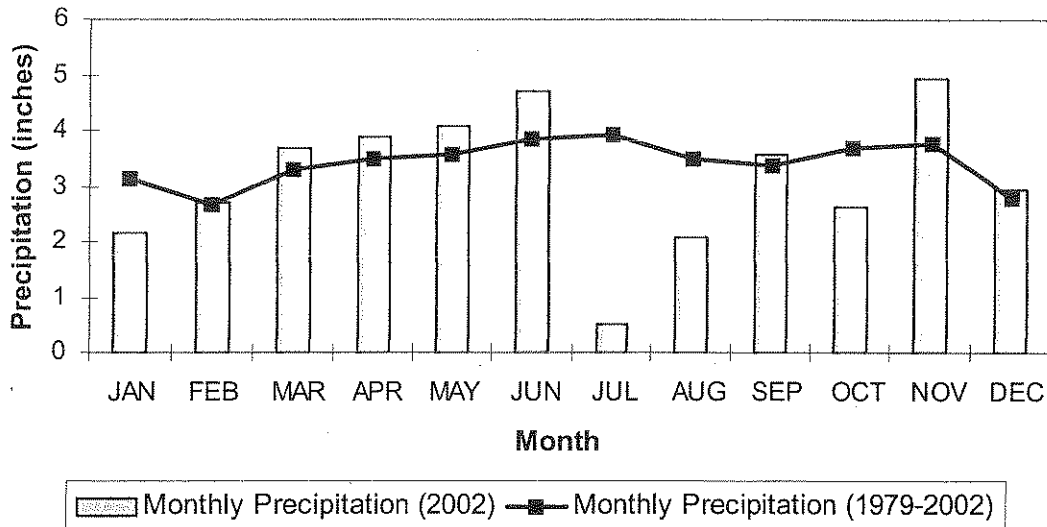
Figure 7: Lakeport 2 Climatological Sampling Station (Laconia, NH) Monthly Precipitation (1979-2002)
