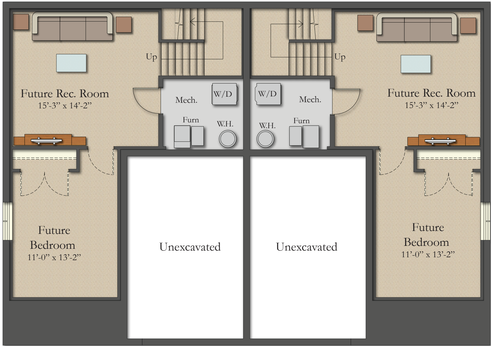
Basement Floor
