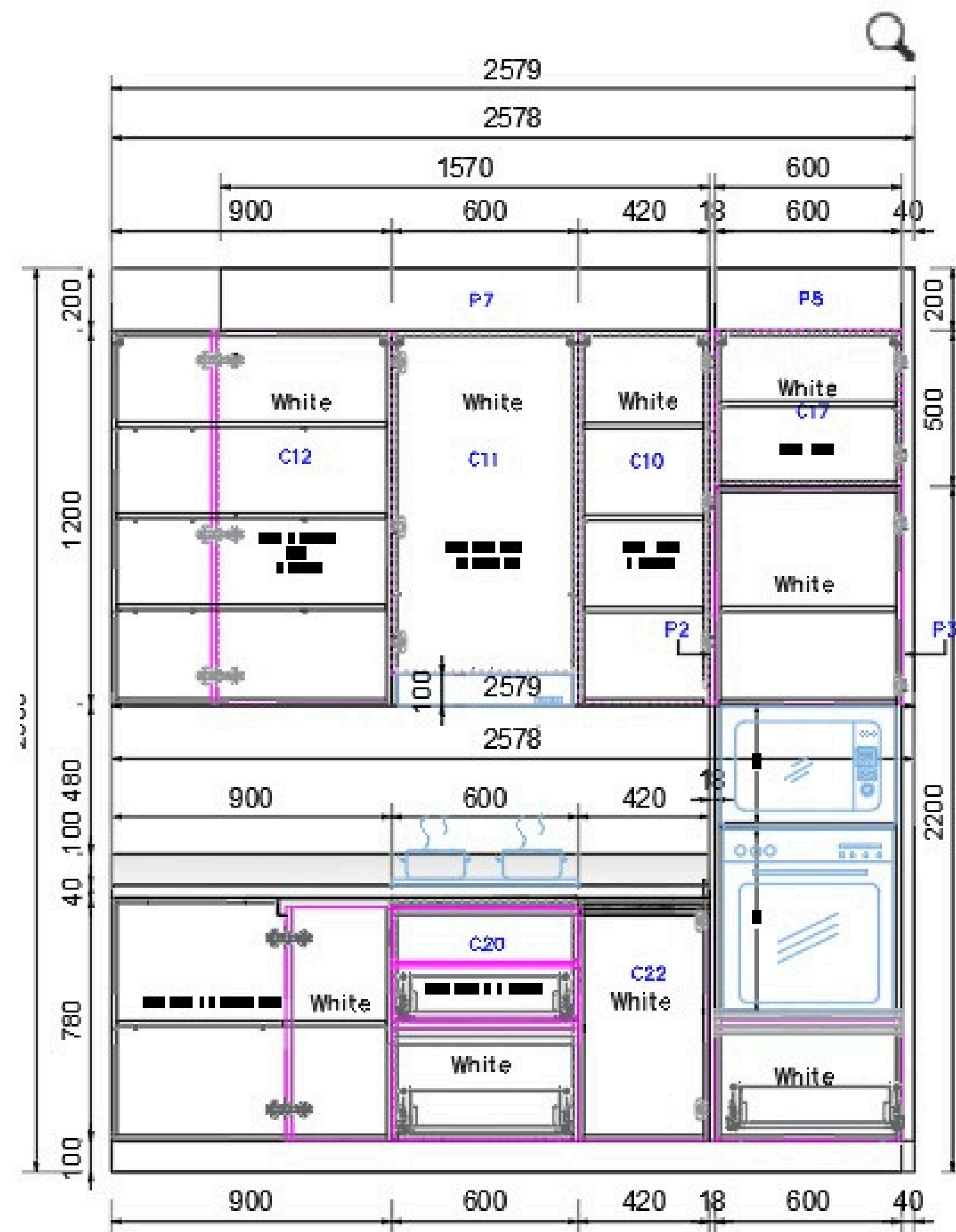
INTERNAL ELEVATION - D
