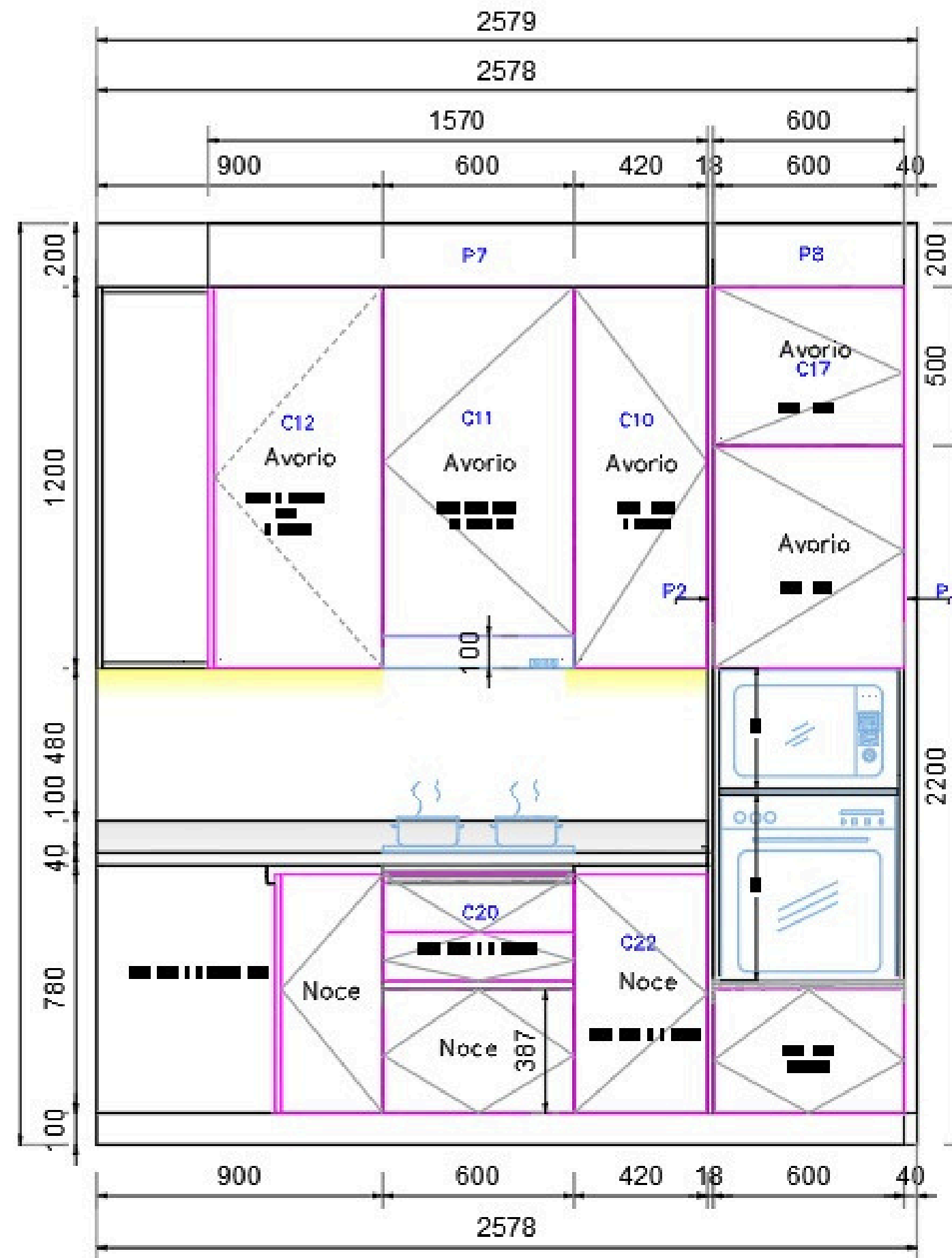
EXTERNAL ELEVATION - D
