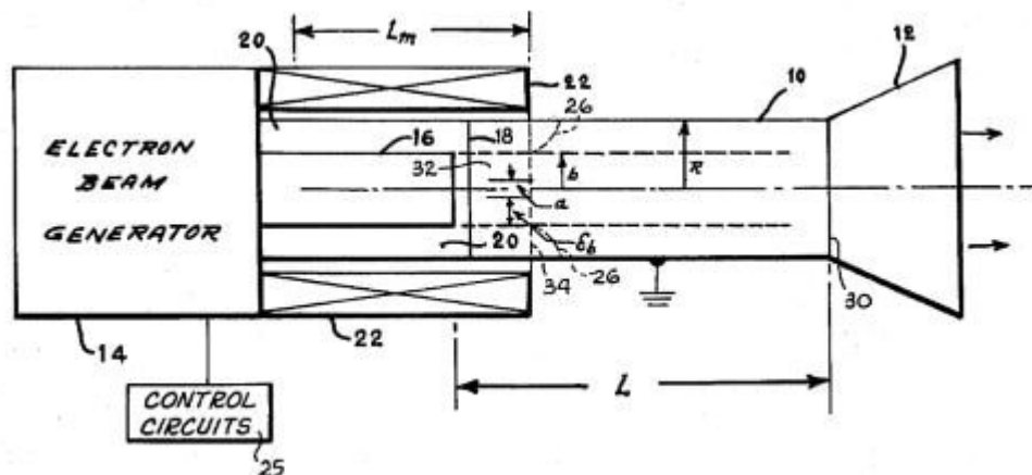
Figure 8. Vircator microwave weapon is mounted on a satellite, and emits a beam that is about 1/2 inch in diameter. The beam travels at the speed of light, and is invisible, just like the microwaves in your oven.
