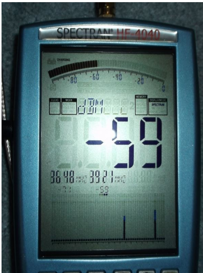
Figure 1. Typical Spectran HF-4040 reading taken in summer 2016. 3648 MHz at -71dbm and 3921 MHz at -59 dbm. There are very few users in this frequency range – so it is easy to identify. Scans were typically done by sweeping between 3500 MHz and 4000 MHz, but could be narrower, once the range is known.
