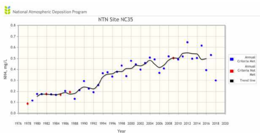
Figure N13. National Atmospheric Deposition Program trend plot for ammonium ion concentration at Clinton monitoring station http://nadp.slh.wisc.edu/data/ntm/plots/ntntrends.html?siteID=NC35
