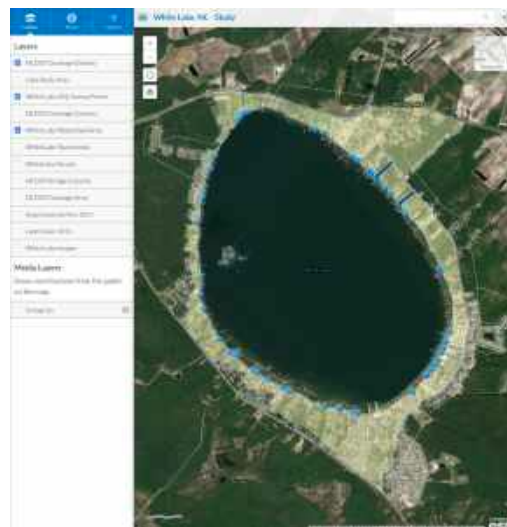
Figure N4. Screen shot of White Lake story map which shows the watershed (in yellow) and the locations of stormwater pipes and ditches which drain to White Lake.
