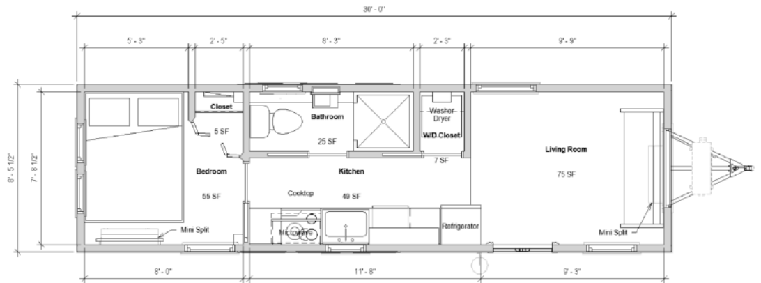
① Main Level Floor Plan 3/8" = 1'-0"
