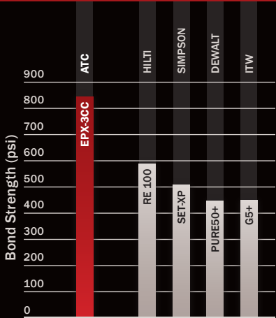
0.500 Inch Diameter Threaded Rod
