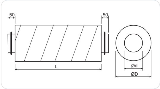
Circular sound attenuator in galvanized steel with insulation shell thickness between 50 and 100 mm
