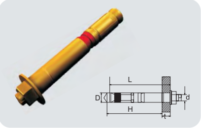
FADE anchor(wedgind)
