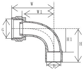
Rotalock valve
