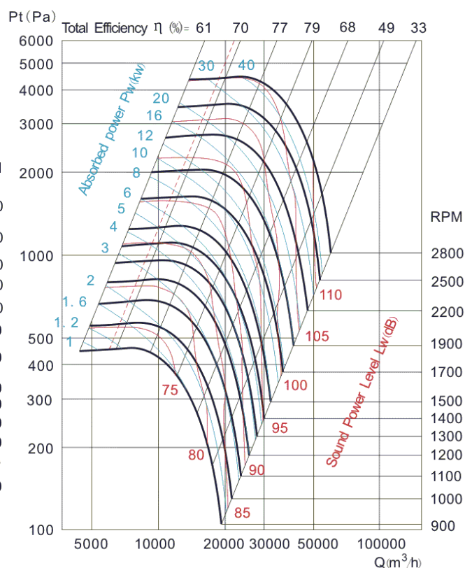
CBA-BS-710BD-X-X-X
