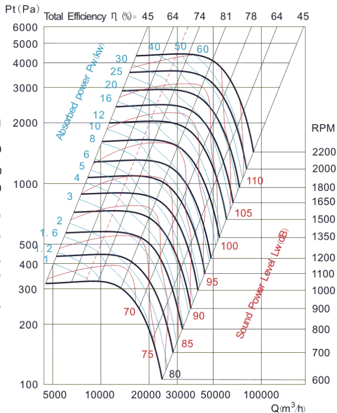
CBA-BS-710BD-X-X-X
