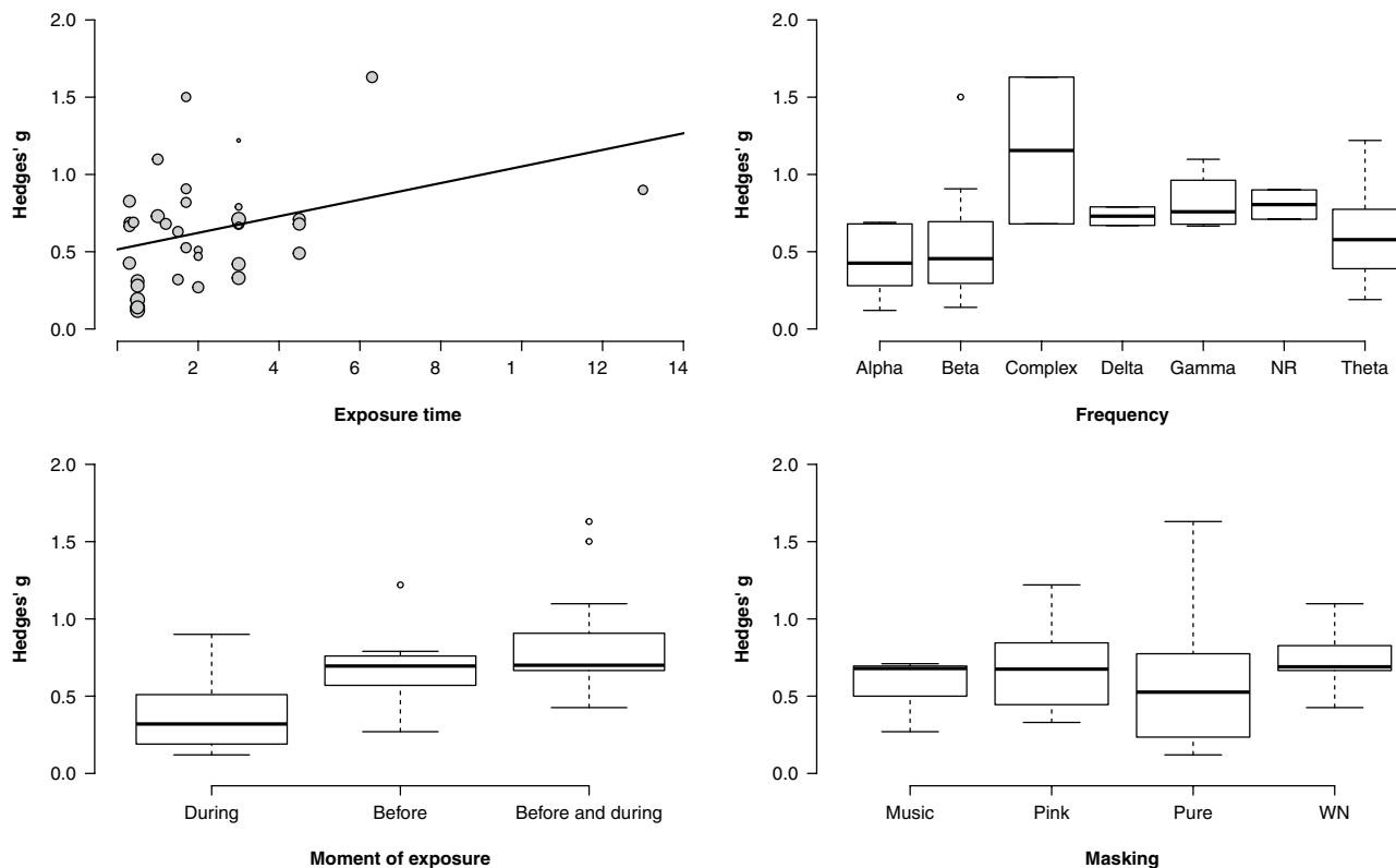
Fig. 9 Box plot of the of exposure time, frequency, moment of exposure, and masking variables. The size of each circle is inversely proportional to the variance ( v ) of each study effect size
