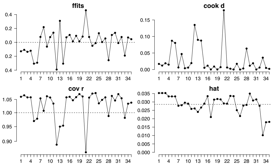
Fig. 2 Plot of four outlier diagnostic statistics for every study; DFFITs difference in standardized fits, cook.d cook’s distance, cov.r ratio of generalized variances, hat leverages or hat values
