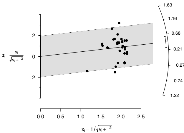
Fig. 6 Galbraith radial plot with 95% CIs of the effects of binaural beats across studies. v variance, y Hedges' g , v_i between-study estimated variance
