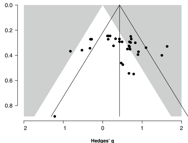
Fig. 4 Funnel plot with pseudo-95% CI of the estimated effect sizes and its standard error in individual studies for the overall studies
