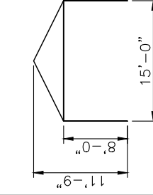
Frame Side View
