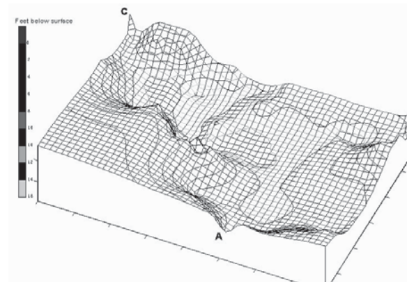
Excavation Mesh Modeling
