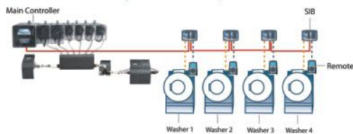
Installation Schematic Diagram of OP Elite Dispensers for 4 washers:
