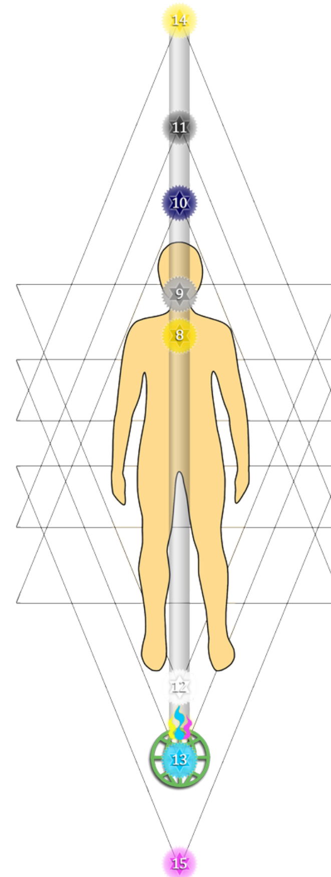
Antiparticle chakras
