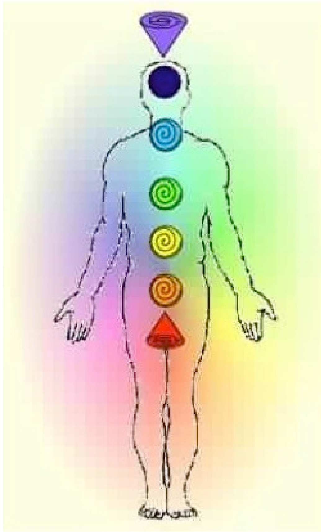
Particle chakras
