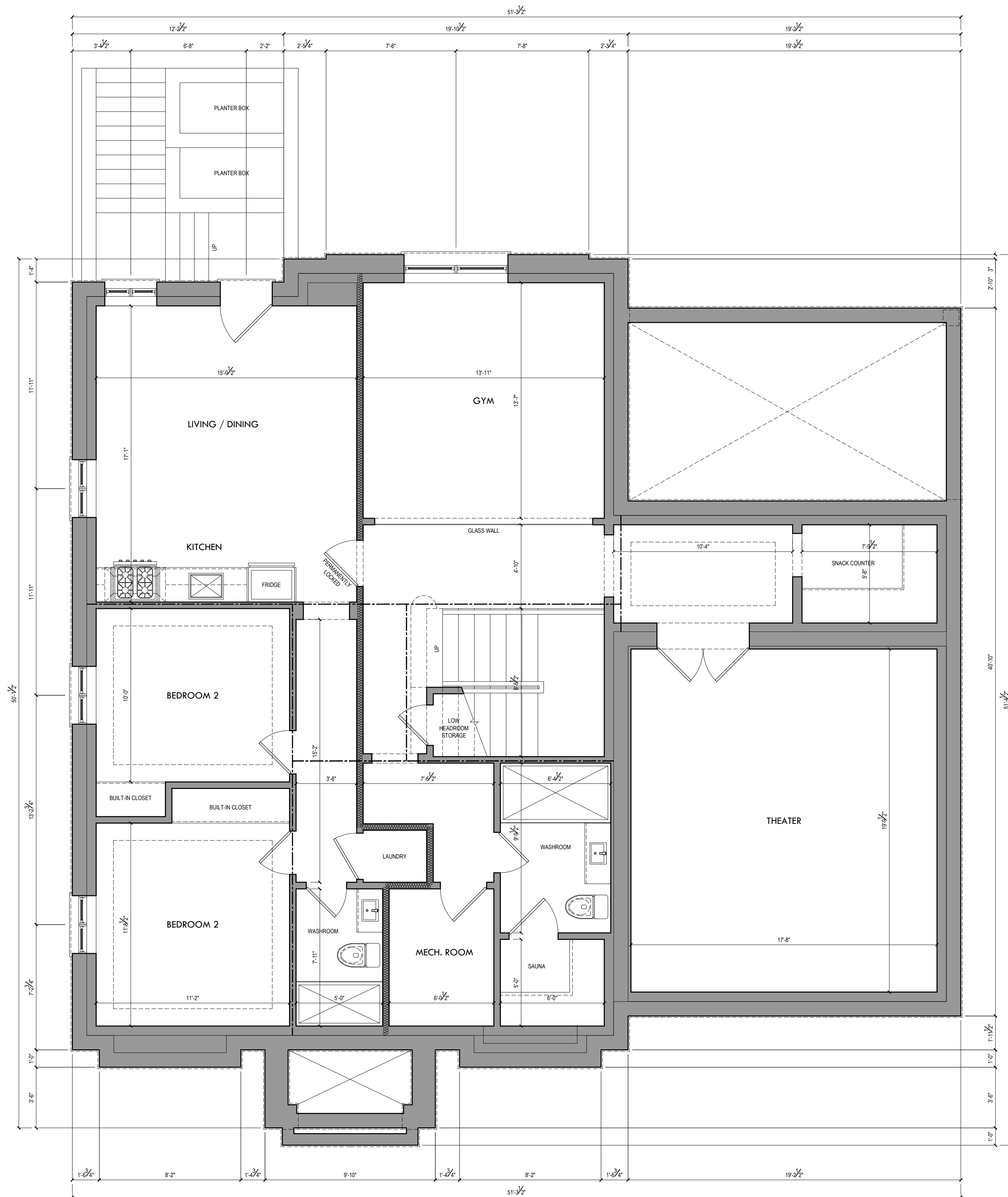
1600 SQ FT BASEMENT FLOOR PLAN
