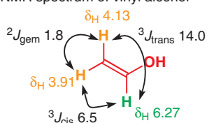
NMR spectrum of vinyl alcohol
