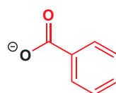
'denatonium benzoate', marked as Bitrex benzyl-diethyl[(2,6-xylyl-carbamoyl)methyl]ammonium benzoate
