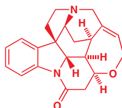
strychnine, or (1R,11R,18S,20S,21S,22S)-12-oxa-8,17-diazaheptacyclo[15.5.0 1,8 .0 2,7 .0 15,20 ]tetracos-2,4,6,14-tetraene-9-one (IUPAC) or 4aR-[4α,5α,8αR*,15α,15bα,15cβ]-2,4a,5,5a,7,8,15,15a,15b,15c-decahydro-4,6-methano-6H,14H-indolo[3,2,1-ij]oxepino[2,3,4-de]pyrrolo[2,3-h]quinolone (Chemical Abstracts)
