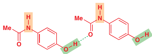
the hydrogen-bonded OH group in paracetamol
