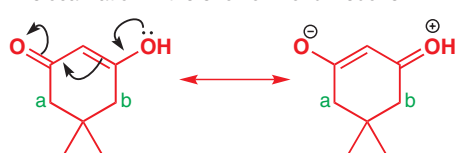
Delocalization in the enol form of dimedone
