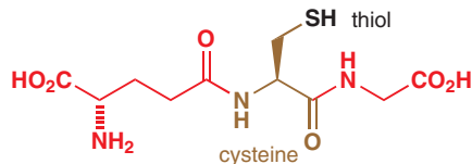
glutathione: scavenger of toxic oxidants
