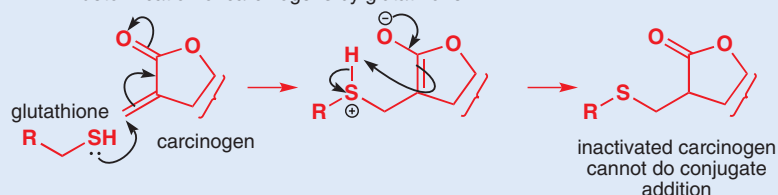
detoxification of carcinogens by glutathione
