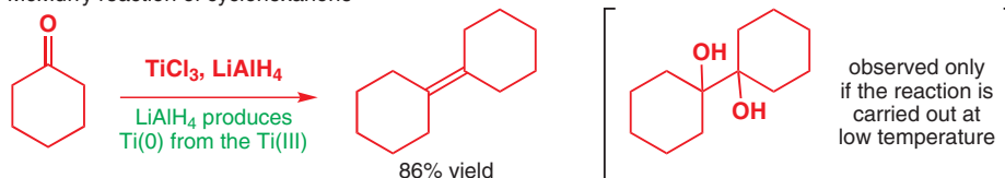
McMurry reaction of cyclohexanone
