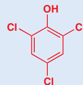
2,4,6-trichlorophenol (TCP)
