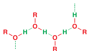
hydrogen bonding in an alcohol
