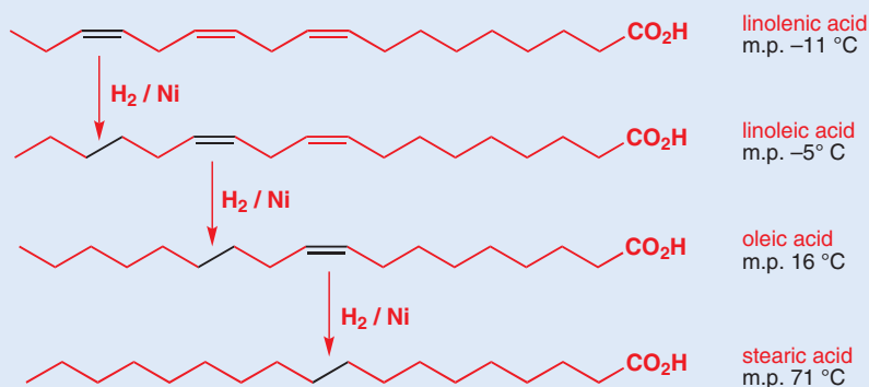
melting points of some common fatty acids
