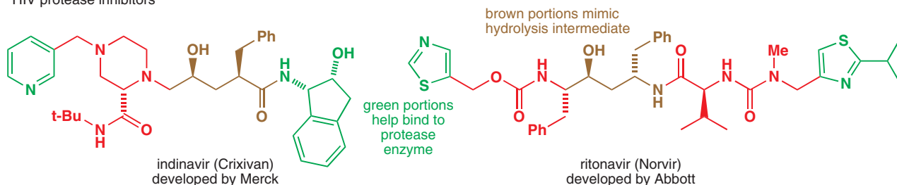
HIV protease inhibitors
