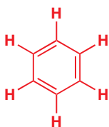
two ways of drawing benzene
