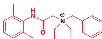
'denatonium benzoate', marked as Bitrex benzyl-diethyl[(2,6-xylyl-carbamoyl)methyl]ammonium benzoate
