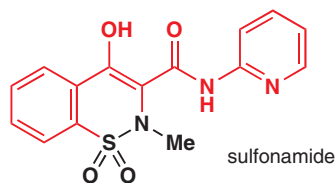
Pfizer's piroxicam or feldene
