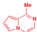
smell of roast meat
