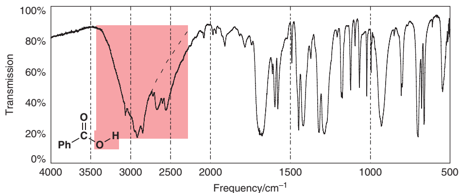
Spectrum 4
