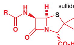
penicillin family of antibiotics
