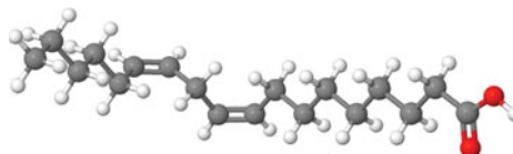
X-ray structure of linoleic acid
