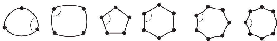
All internal angles 109.5^\circ
