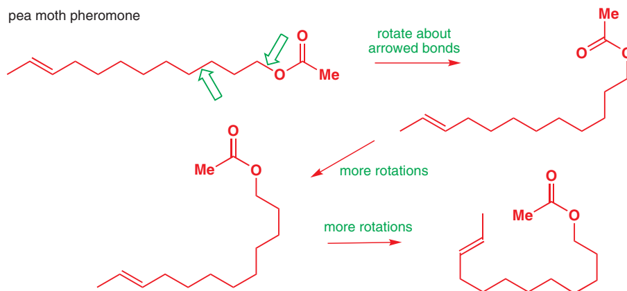
pea moth pheromone
