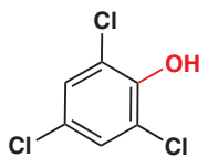
2,4,6-trichlorophenol
