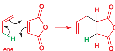
the Alder ene reaction
