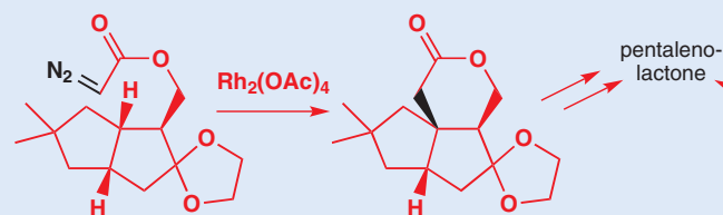
route 1: Cane's synthesis of pentalenolactone
