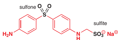
dapsone: water-soluble 'pro-drug' for leprosy
