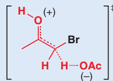
transition state for proton removal
