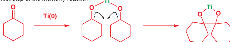
first step of the McMurry reaction
