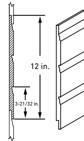
TwelveFour Cottage Lap 7/8 in. Groove 1/2 in. Lap Siding 14.67 sq. ft. coverage/piece
