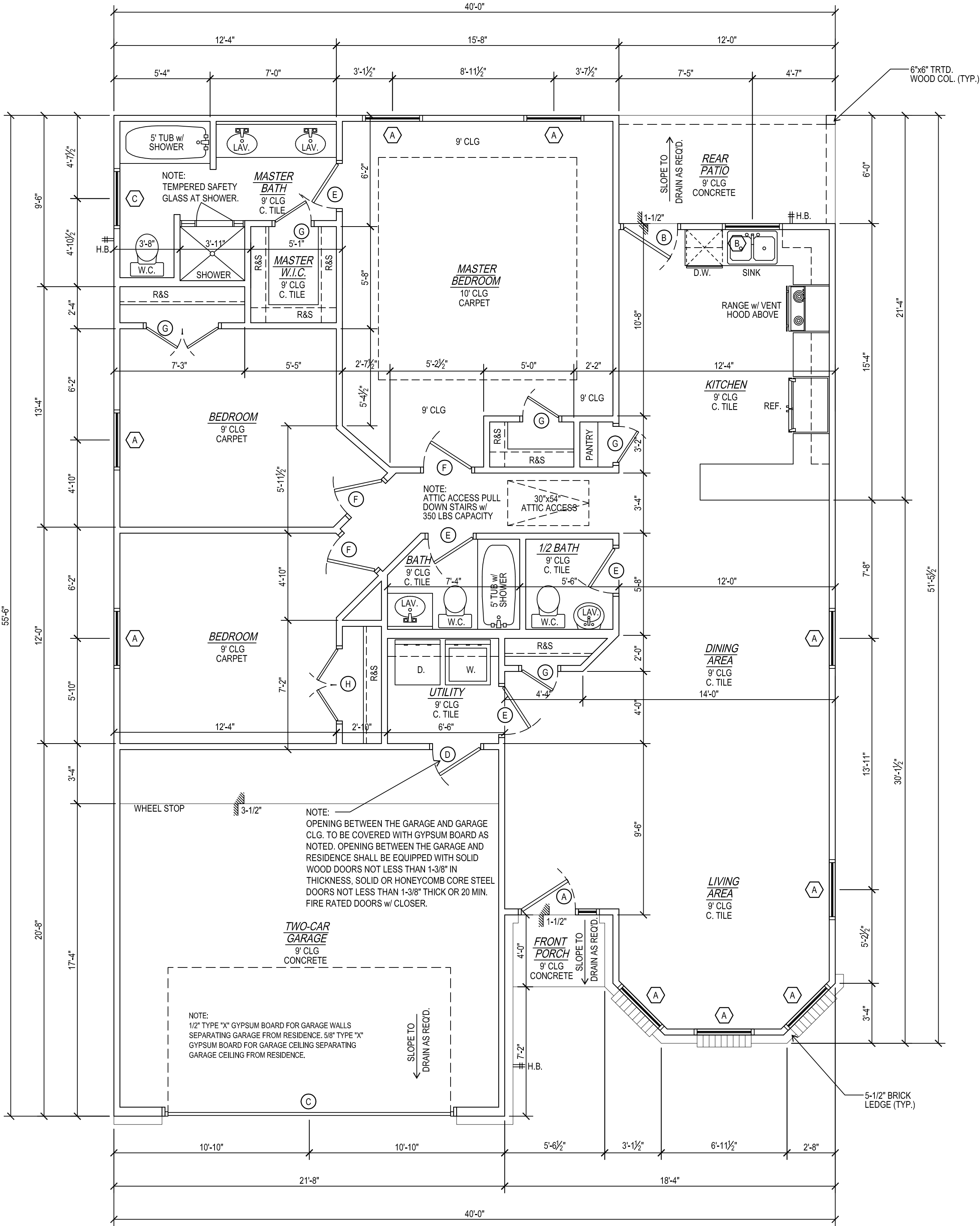
FLOOR PLAN
