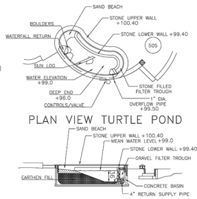
5.2 TURTLE POND: SECTION SCALE: 3/16" = 1'-0"
