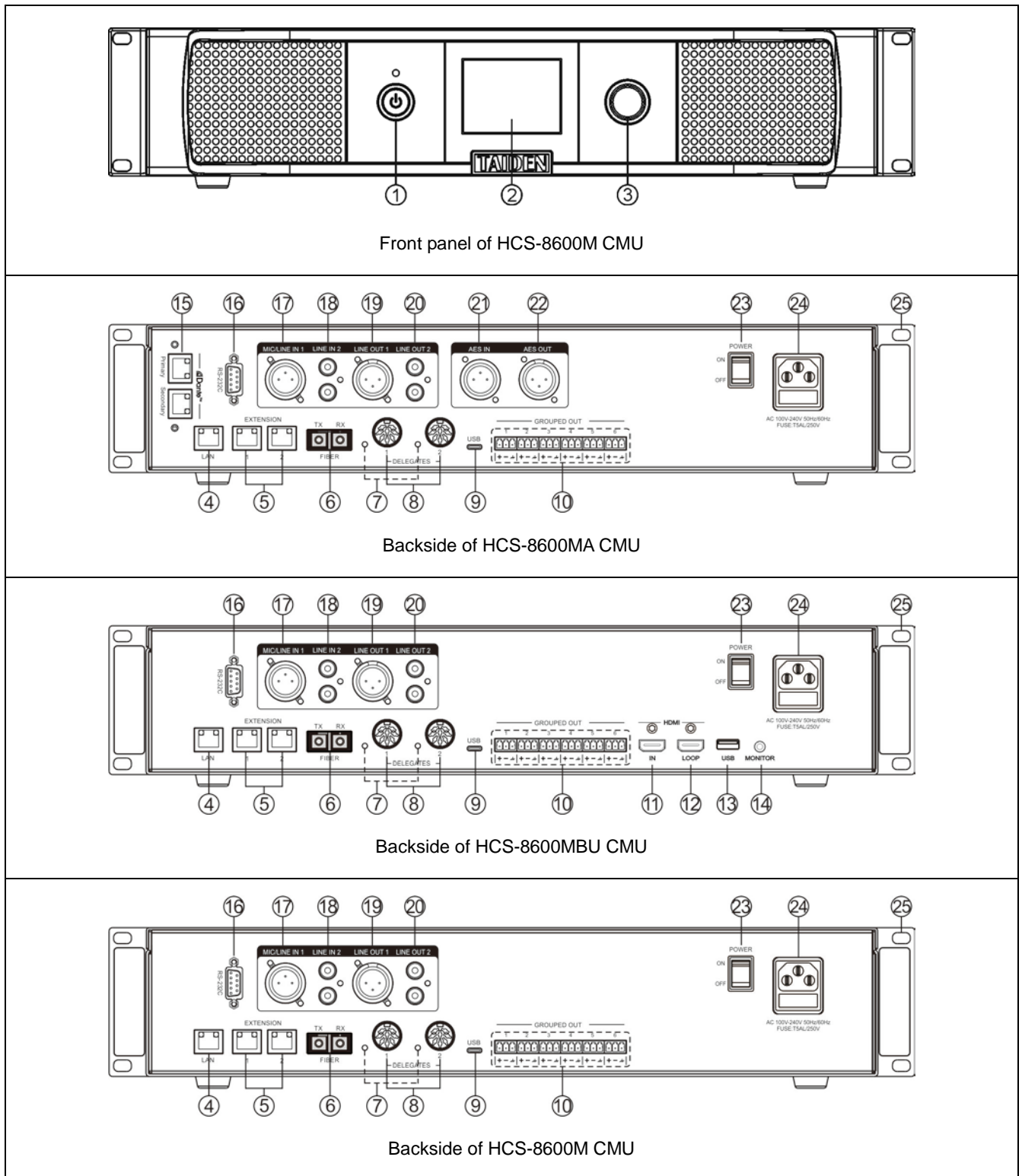
Figure 2.1.1 HCS-8600M series congress main unit
