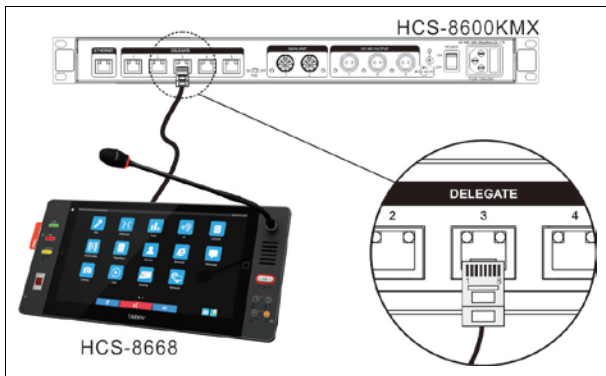
Figure 3.2.5 HCS-8668/8638 series paperless multimedia congress terminal connecting to HCS-8600KMX Ethernet switcher (PoE)
