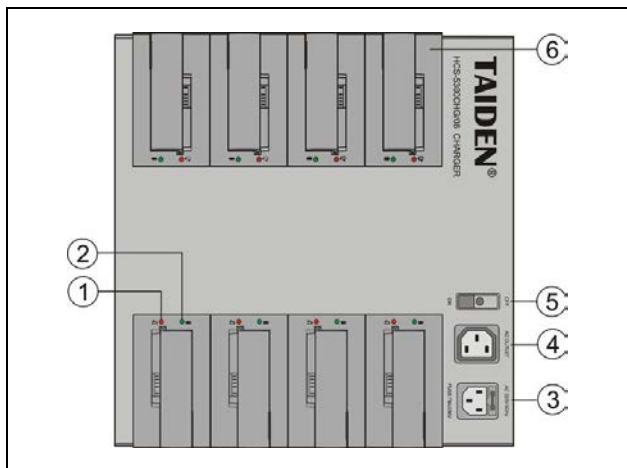
Figure 6.9 HCS-5300CHG/08 charging unit
