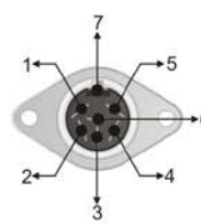
Socket (rear view)
