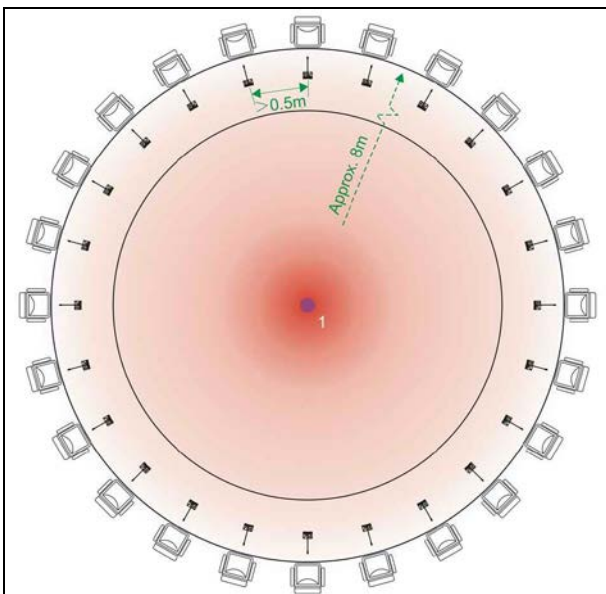
Figure 3.13 Planning the transceiver (round table arrangement)
