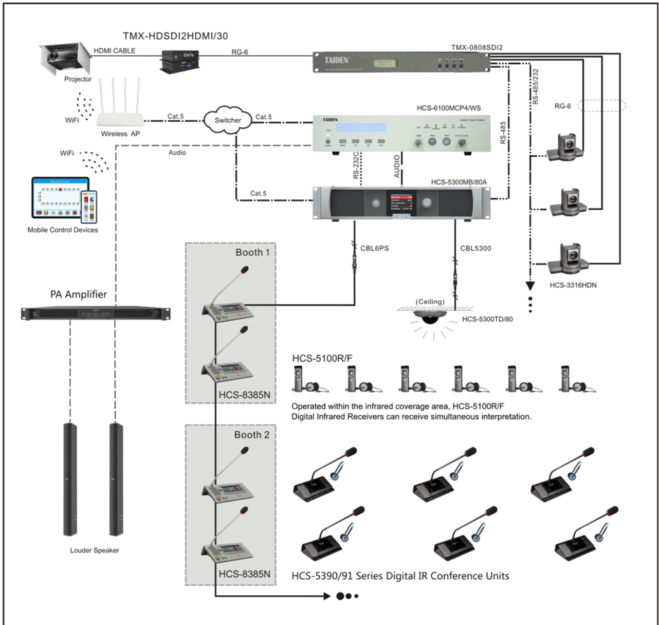
Figure 2.12 System connection [Wired/wireless discussion + digital simultaneous interpretation + video tracking + central control]
