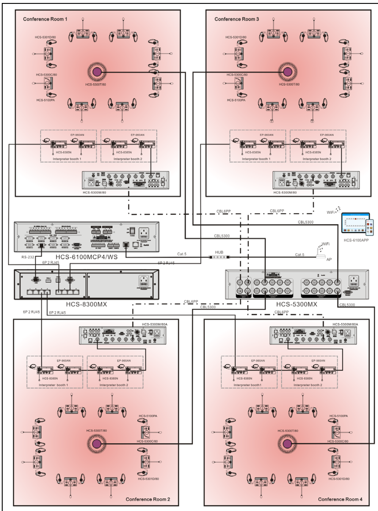
Figure 6.3 Conference rooms combination 2
