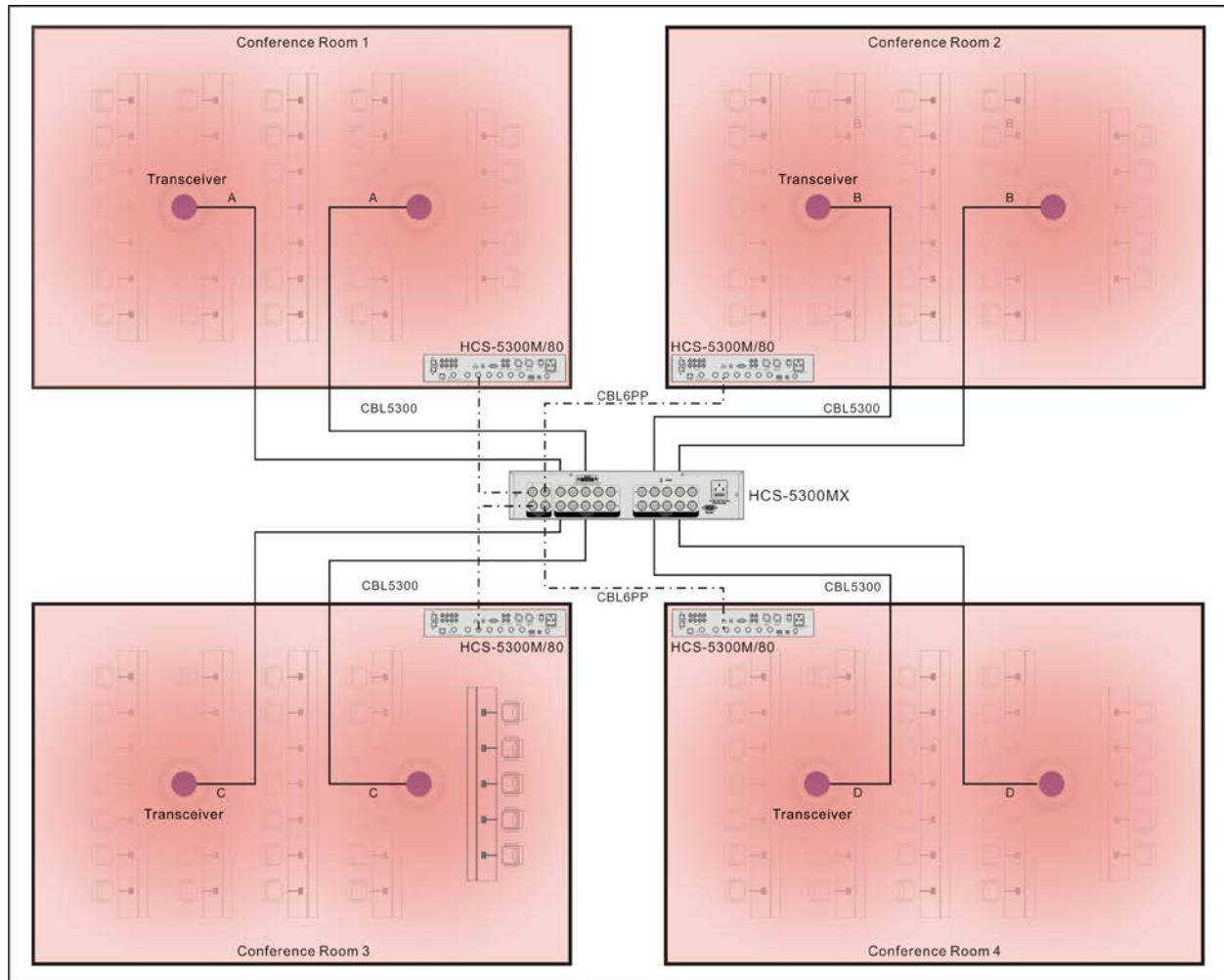
Figure 6.2 Room Combination 1
