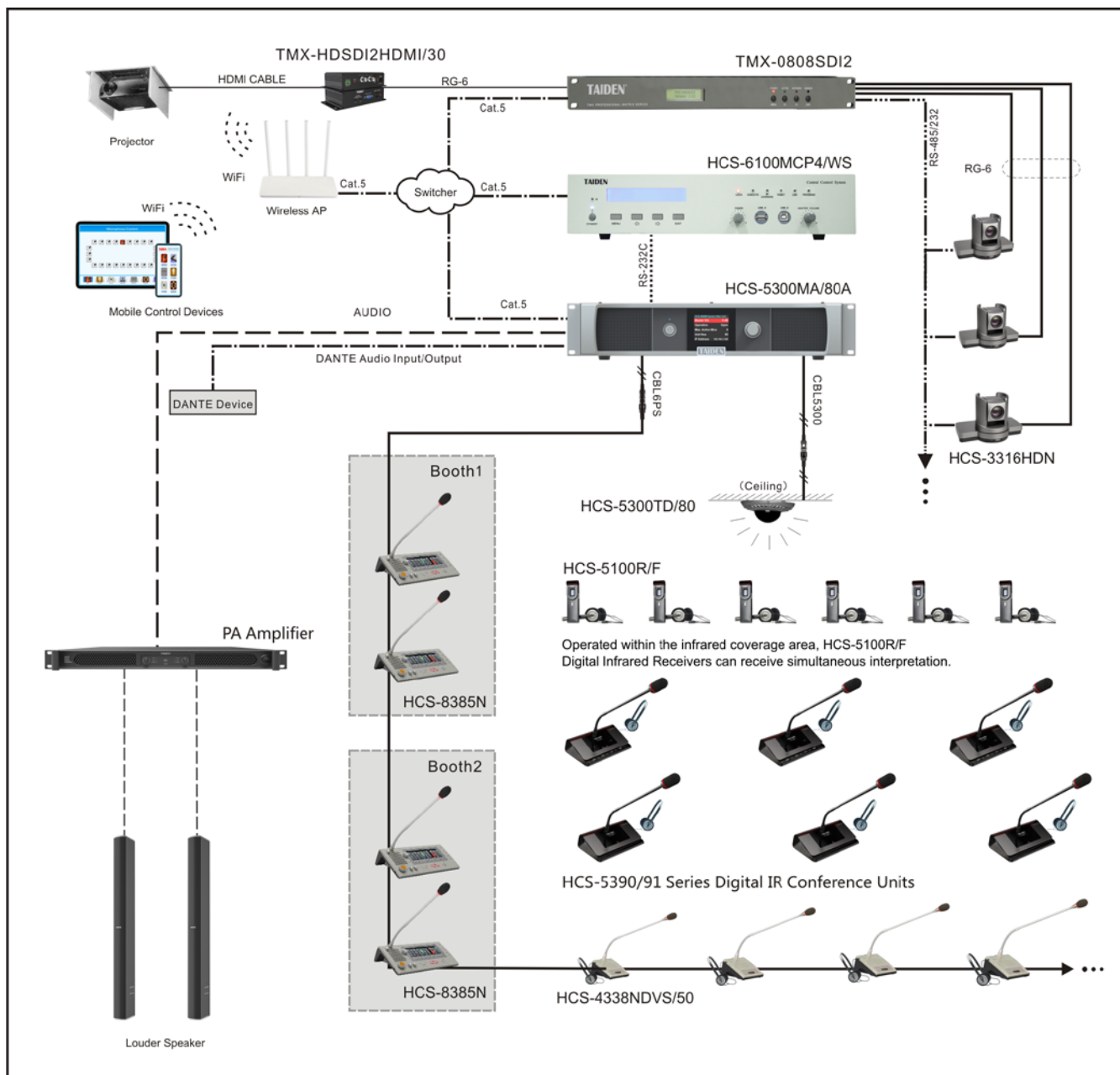
Figure 2.11 System connection [Wired/wireless discussion + digital simultaneous interpretation + voting + video tracking]
