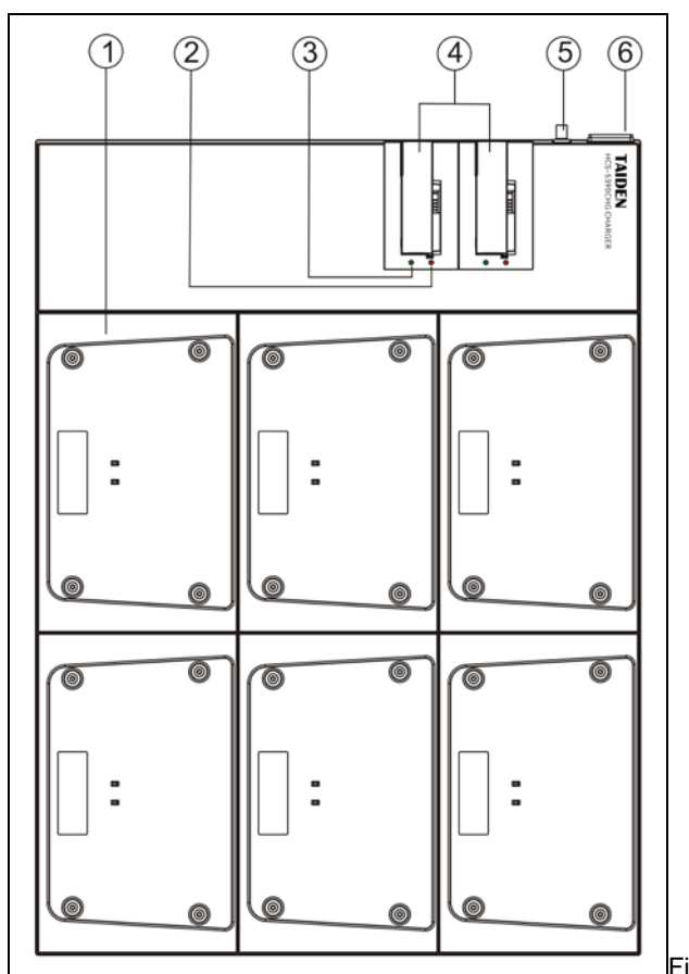
Figure 6.10 HCS-5390CHG charging unit
