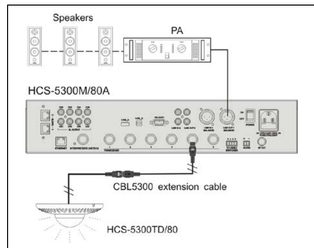
Figure 2.7 Digital infrared wireless conference main unit connecting to PA
