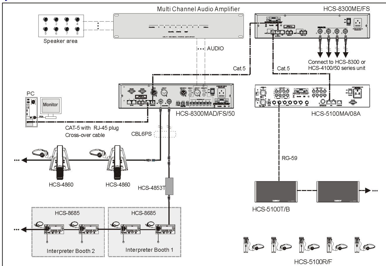
Figure Connection with HCS-8300 series Congress Main unit
