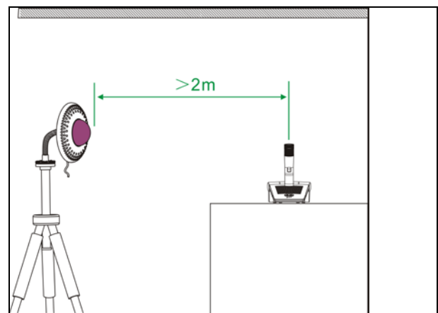
Figure 6.5 Distance between conference unit and transceiver
