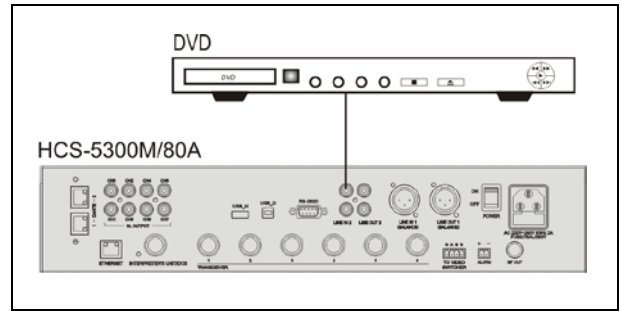
Figure 2.5 Main unit connecting to external audio device through "LINE IN" interface
