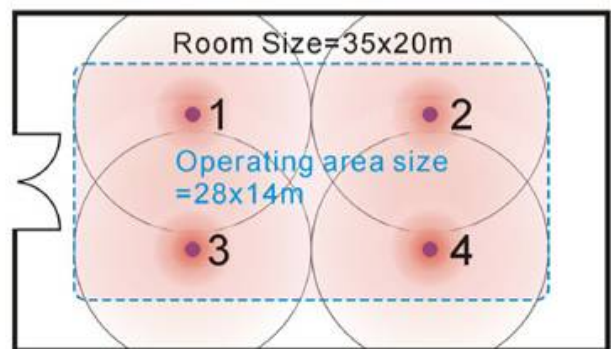
Figure 3.11 Four transceivers cover the whole operating area
