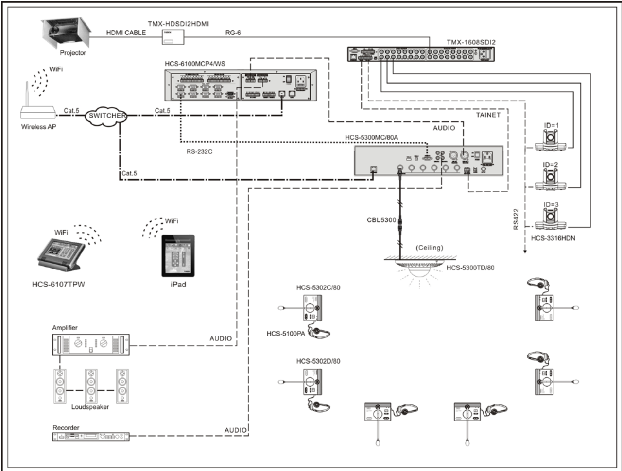
Figure 2.11 System connection [Wireless discussion + video tracking + central control]
