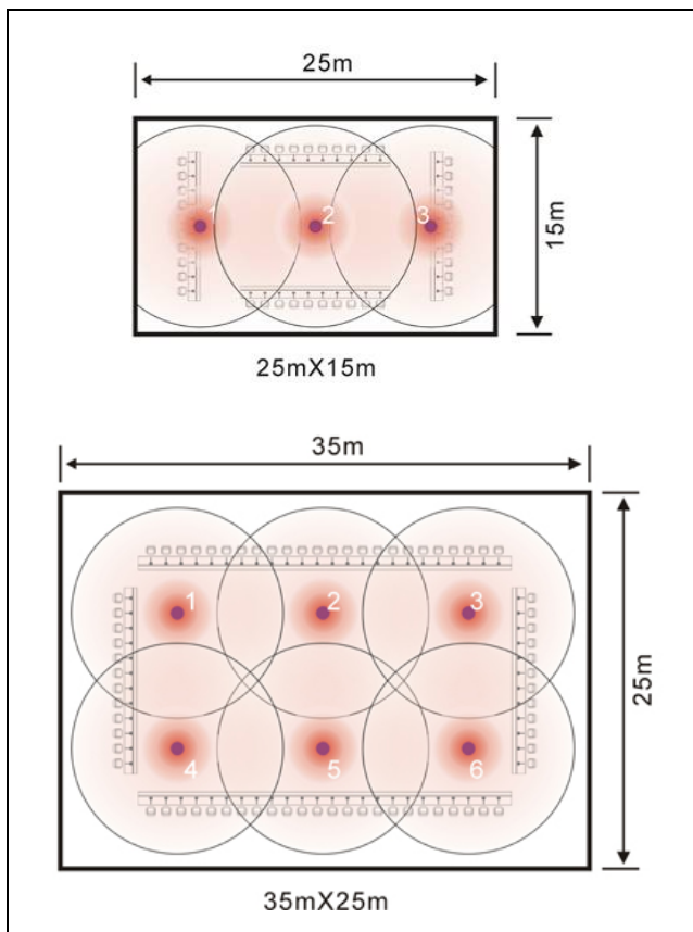
Figure 3.15 Planning the transceiver (conference style seating)
