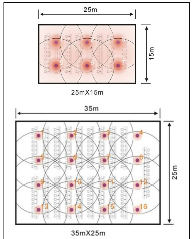
Figure 3.17 Planning the transceiver (parliamentary seating)
