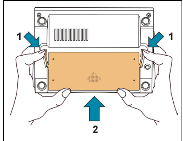
Figure 8.6 Disassemble HCS-5300BAT battery
