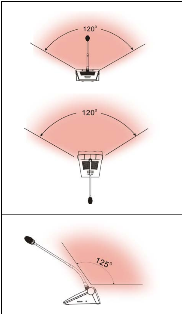
Figure 5.2 Coverage area of digital infrared wireless conference unit
