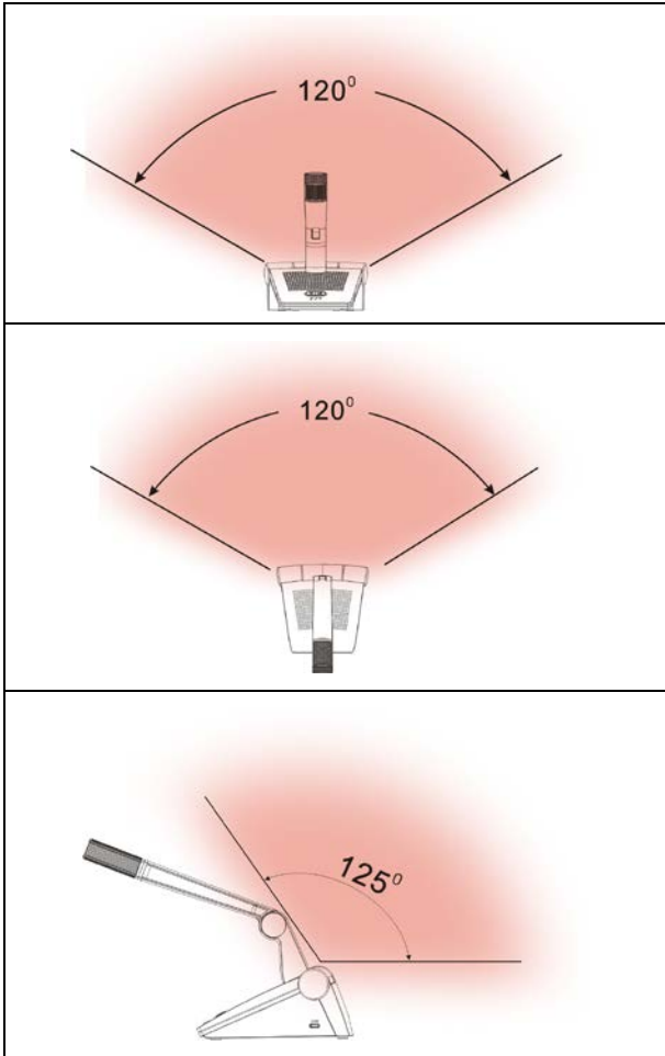
Figure 6.2 Coverage area of digital infrared wireless conference unit
