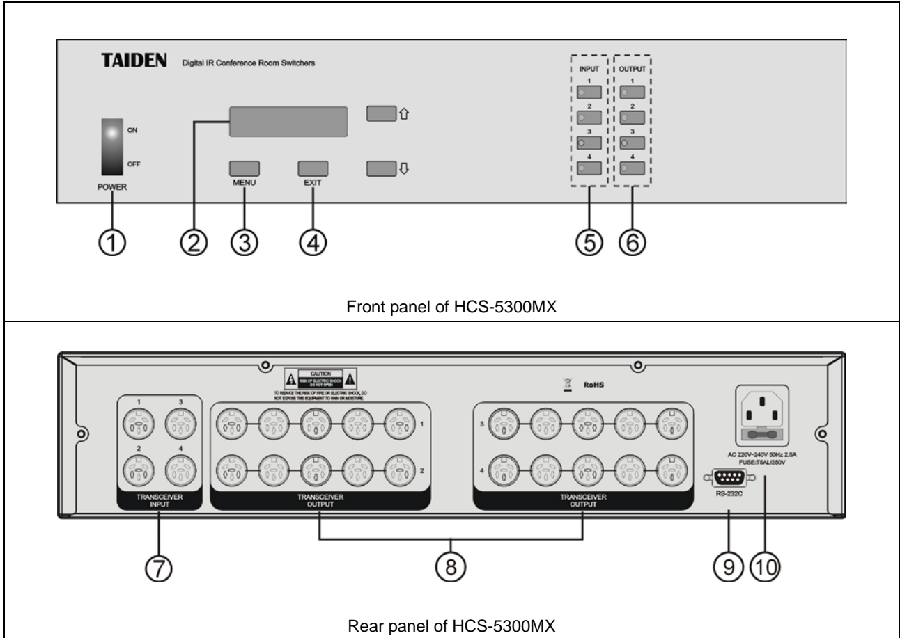
Figure 8.1 HCS-5300MX Digital IR Conference Room Switcher
