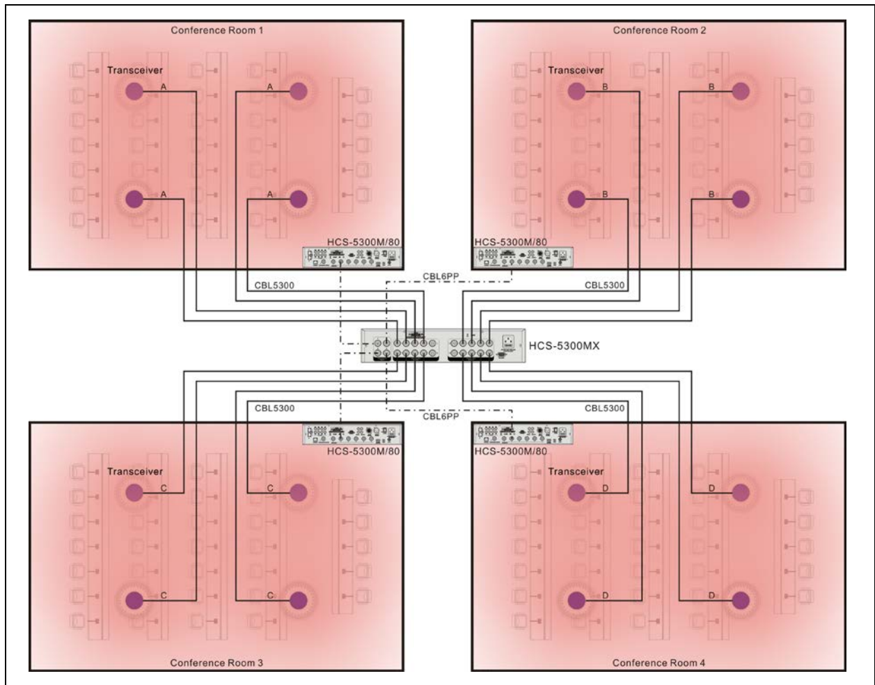
Figure 8.2 Splitting/Combining several meeting rooms 1
