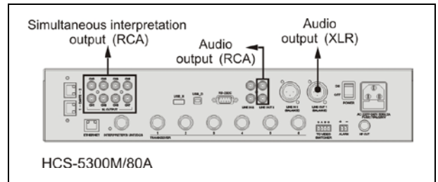
Figure 2.6 Main unit connecting to recording device
