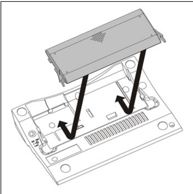
Figure 8.5 Assemble HCS-5300BAT battery
