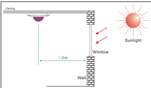
Figure 3.4 Digital infrared transceiver/receiver position (near window)
