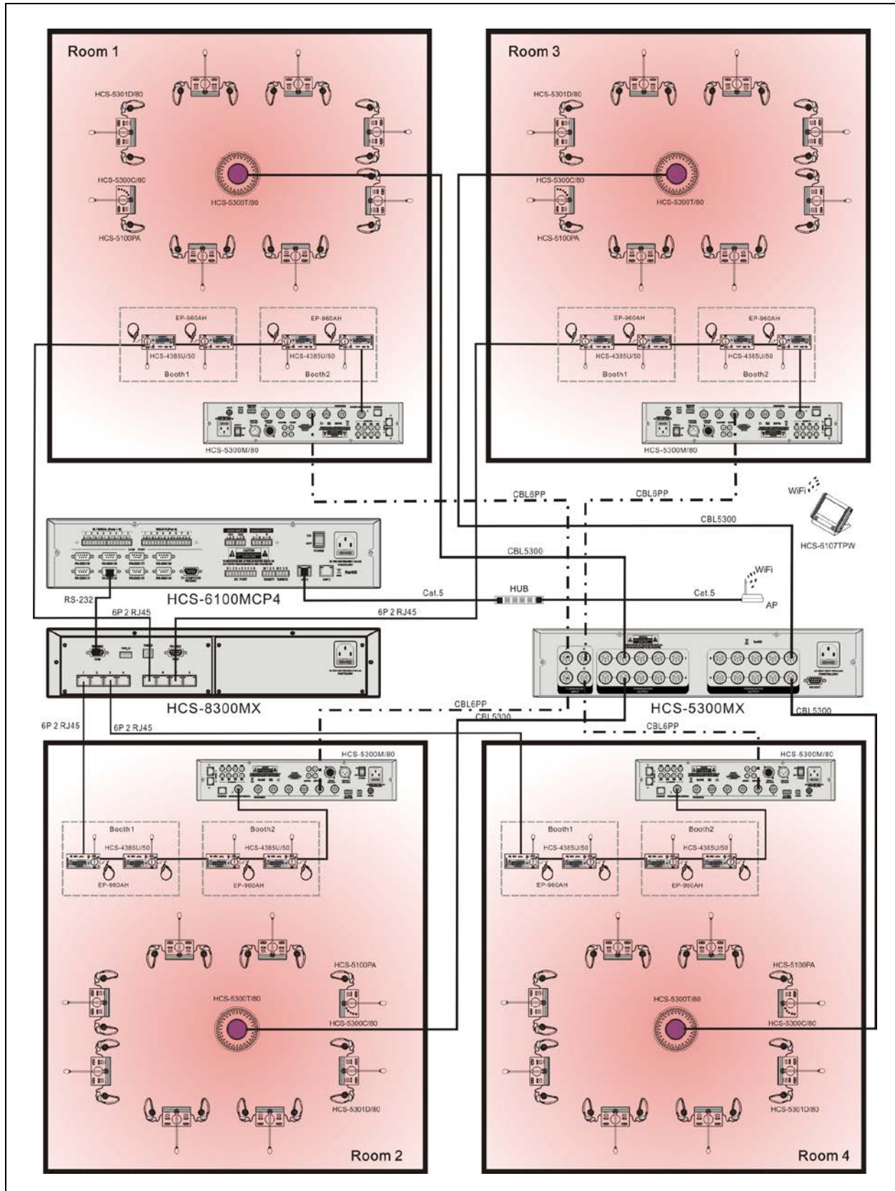
Figure 8.3 Splitting/Combining several meeting rooms
