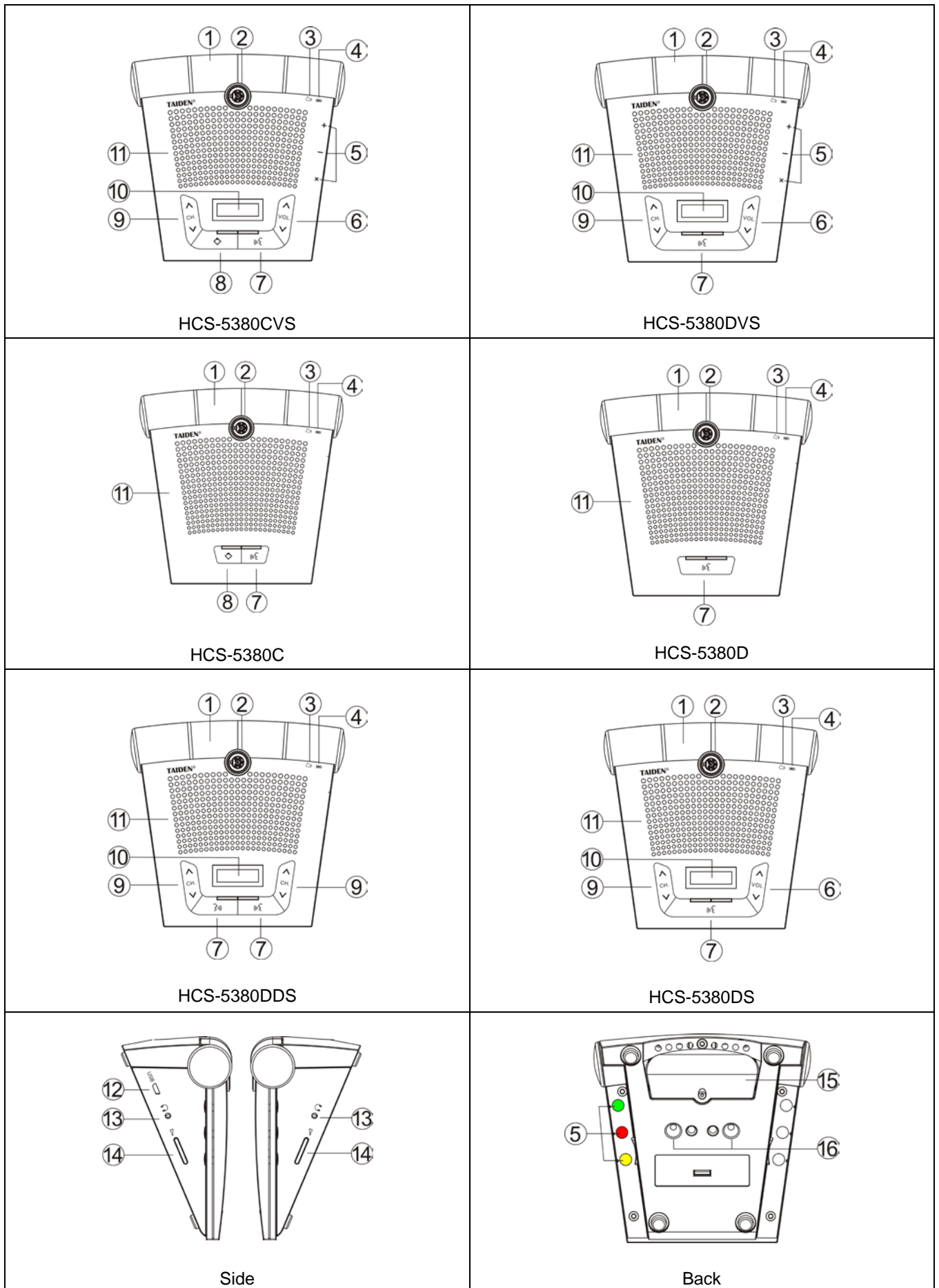
Figure 5.1 HCS-5380 series digital infrared wireless conference unit
