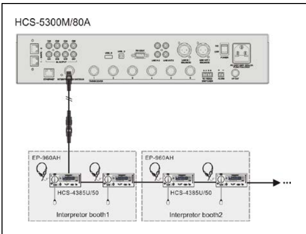
Figure 2.4 Main unit connecting to HCS-4385U/50 through interpreter's unit interface
