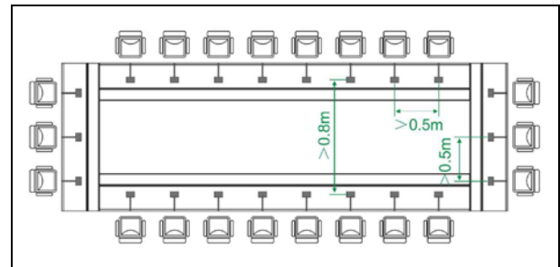
Figure 5.4 Distance between conference units
