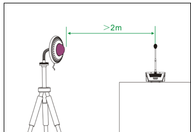
Figure 5.5 Distance between conference unit and transceiver
