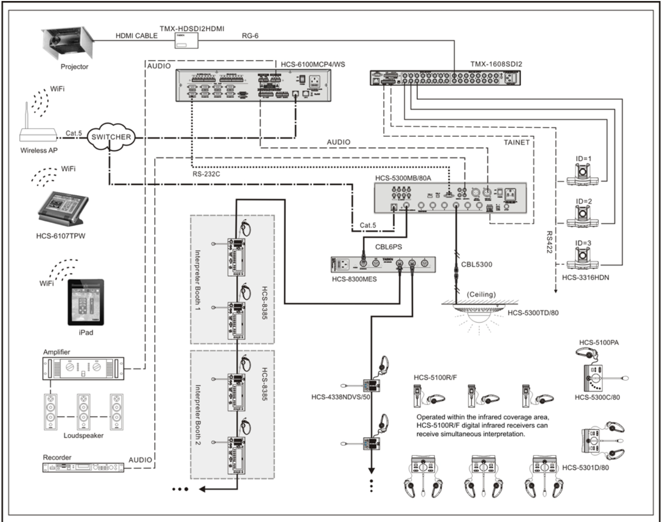
Figure 2.10 System connection [Wired/wireless discussion + digital simultaneous interpretation + video tracking + central control]
