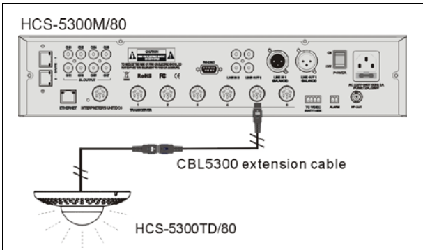
Figure 3.31 Digital infrared transceiver connecting to digital infrared wireless conference main unit
