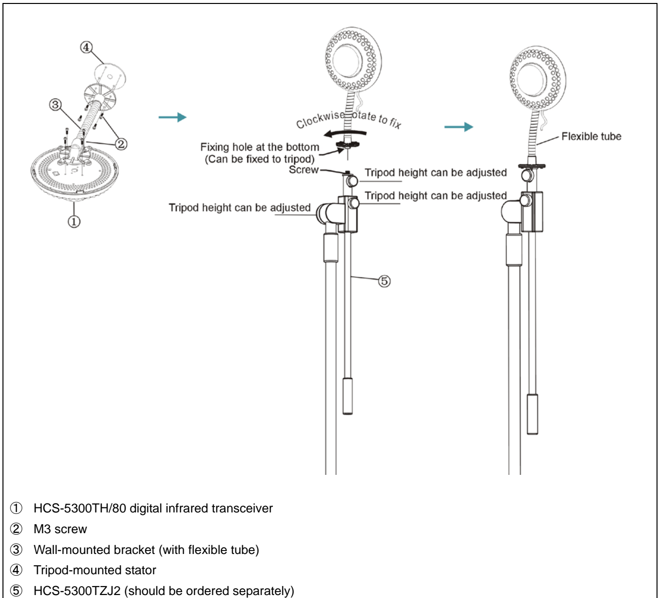
Figure 3.29 HCS-5300TH/80 digital infrared transceiver tripod mounted
