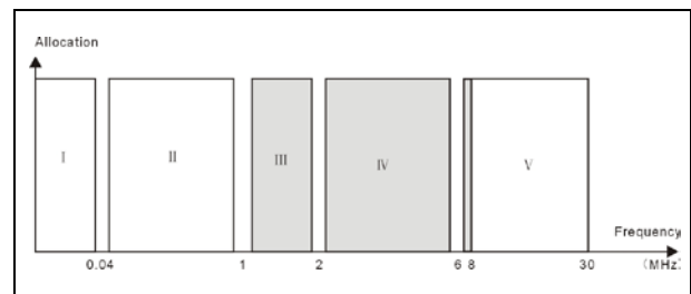
Figure 1.3 Standard wave band in HCS-5300/80 system
