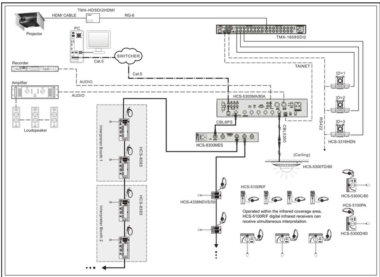
Figure 2.9 System connection [Wired/wireless discussion + digital simultaneous interpretation + voting + video tracking]
