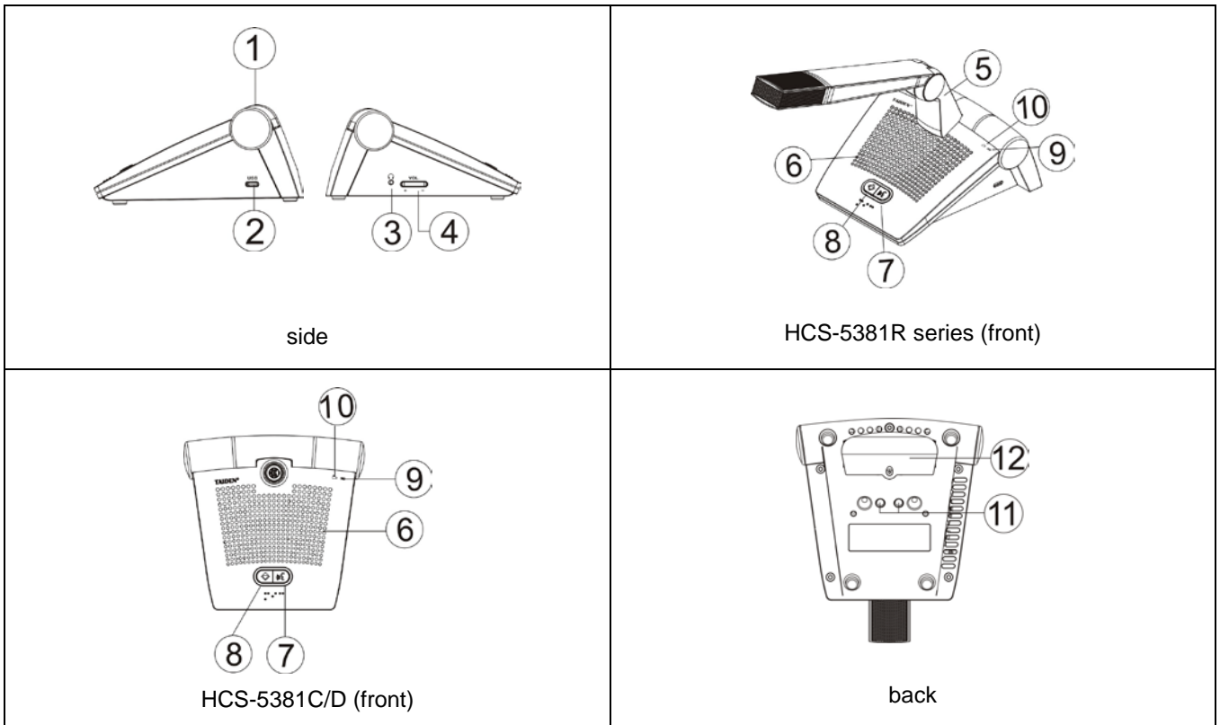
Figure 6.1 HCS-5381 series digital infrared wireless conference unit
