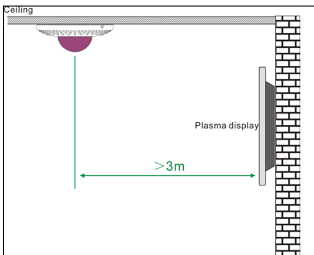
Figure 3.8 Digital infrared transceiver/receiver position (near plasma display)
