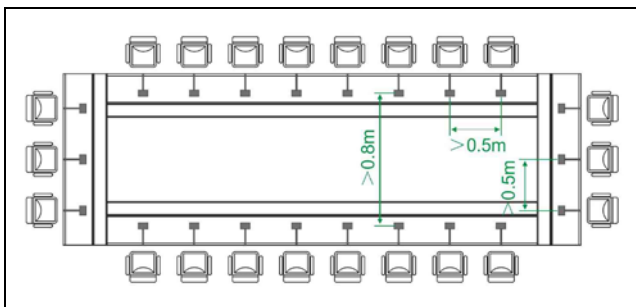
Figure 4.4 Distance between conference units
