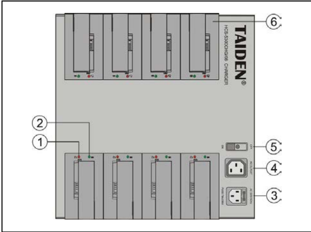
Figure 8.7 HCS-5300CHG/08 charging unit
