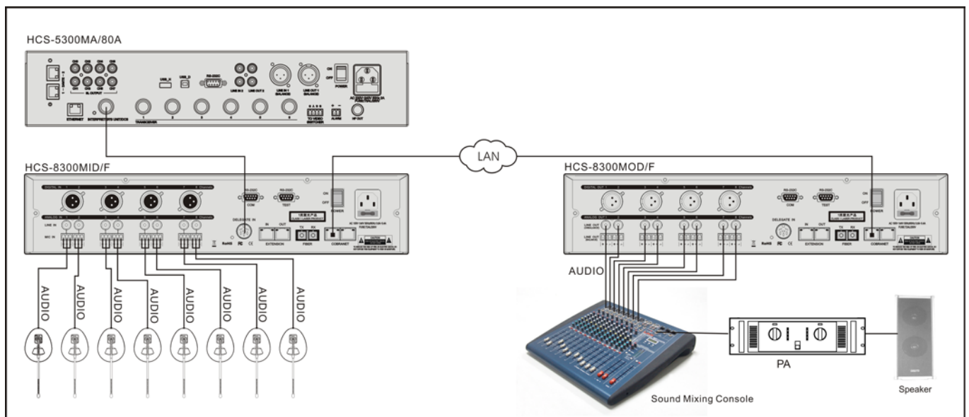
Figure 2.8 HCS-5300M+HCS-8300MI+HCS-8300MO multi-channel digital audio transmission solution
