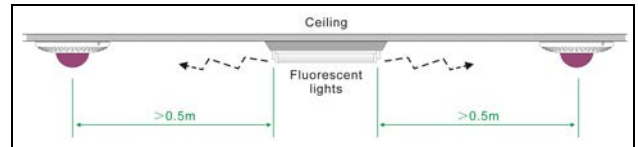
Figure 3.5 Digital infrared transceiver/receiver position (near lighting equipment)
