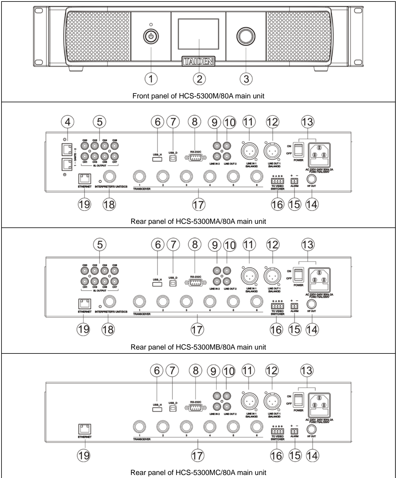
Figure 2.1 Digital infrared wireless conference system main unit
