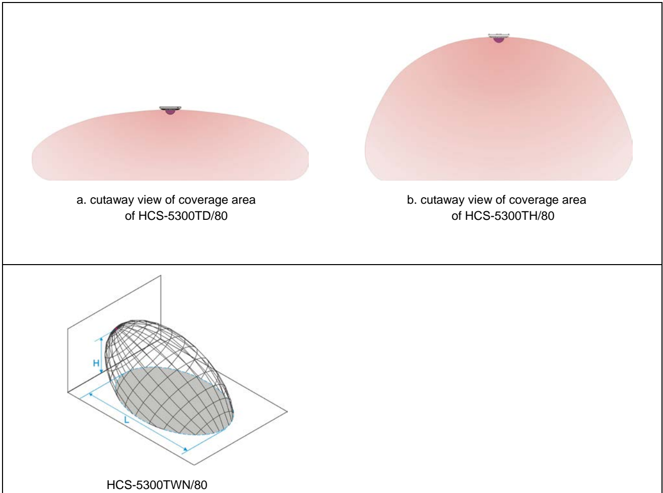
Figure 1.7 Coverage area of digital infrared transceiver
