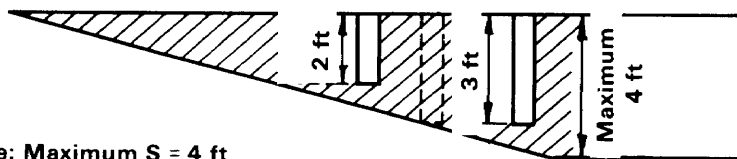
SECTION
