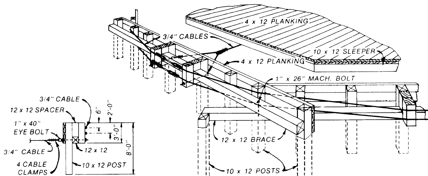
ASSEMBLY PICTORIAL
