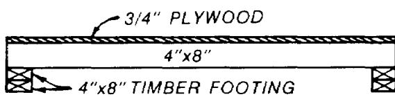
ROOF DETAIL
