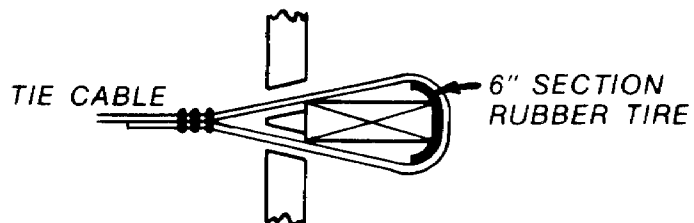
ALTERNATE TIE CABLE ATTACHMENT
