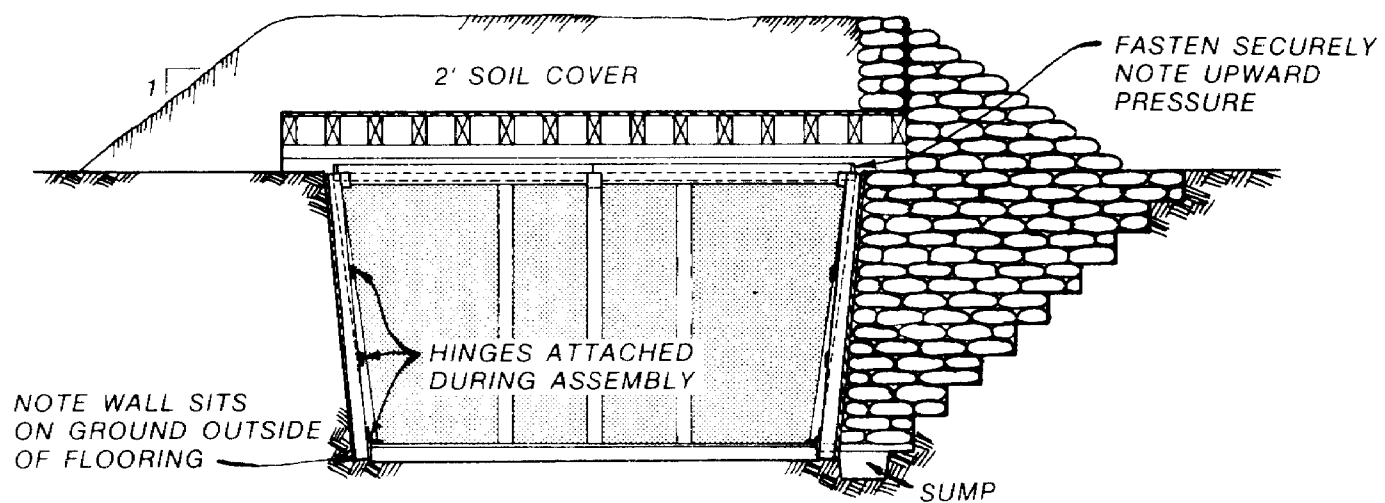
SECTION
