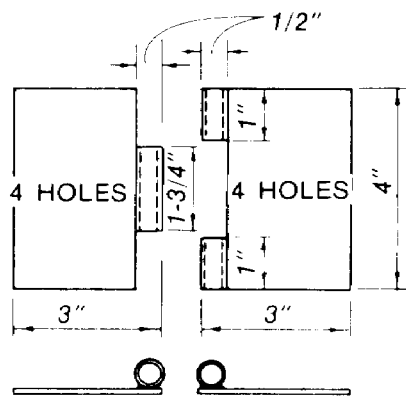
HINGE 16 NEEDED
