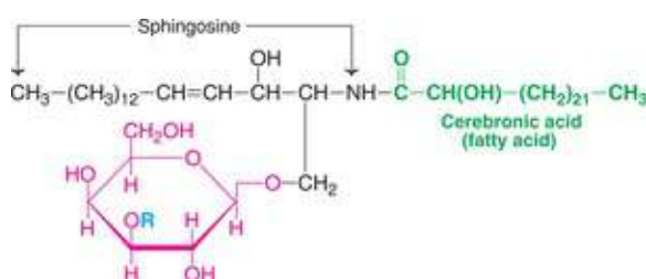
FIG. 3.4 Structure of galactosylceramide (R = H). For sulfagalactosylceramide R is a sulfatide . ( R = \text{SO}_4^{2-} )
