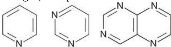
Pyridine
