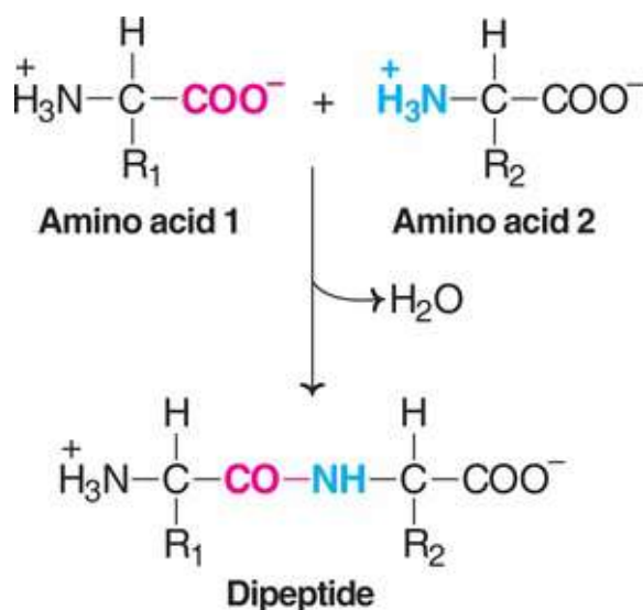
FIG. 4.5 Formation of a peptide bond.
