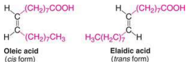
FIG. 3.1 Cis-trans isomerism in unsaturated fatty acids.
