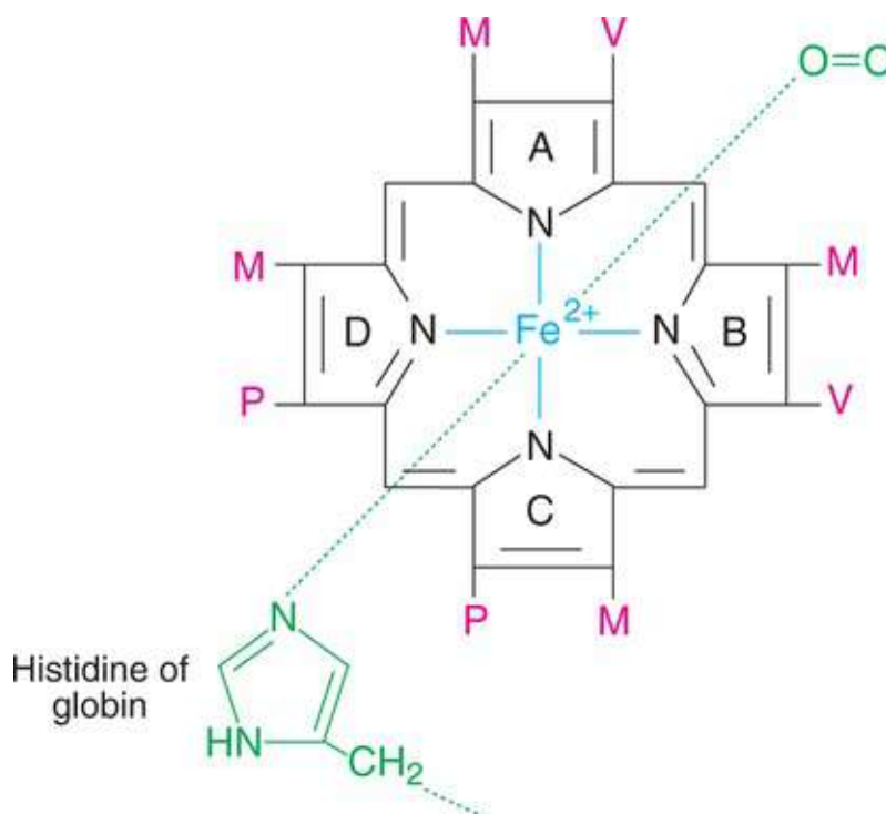
FIG. 10.2 Structure of heme [M-Methyl (–CH 3 ); V-Vinyl (–CH 2 –CH 2 –); P-Propionyl (–CH 2 –CH 2 –CH 2 –)].
