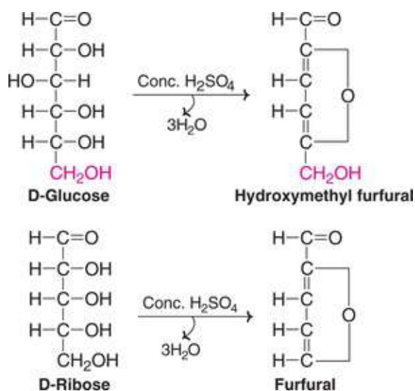
FIG. 2.9 Dehydration of monosaccharides with concentrated \text{H}_2\text{SO}_4 .
