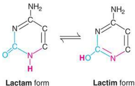
FIG. 5.3 The tautomeric forms of cytosine.
