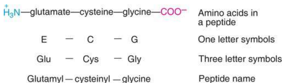
FIG. 4.6 Use of symbols in representing a peptide (Note : A tripeptide with 3 amino acids and two peptide bonds is shown; Free \text{—NH}_3^+ is on the left while free \text{—COO}^- is on the right).
