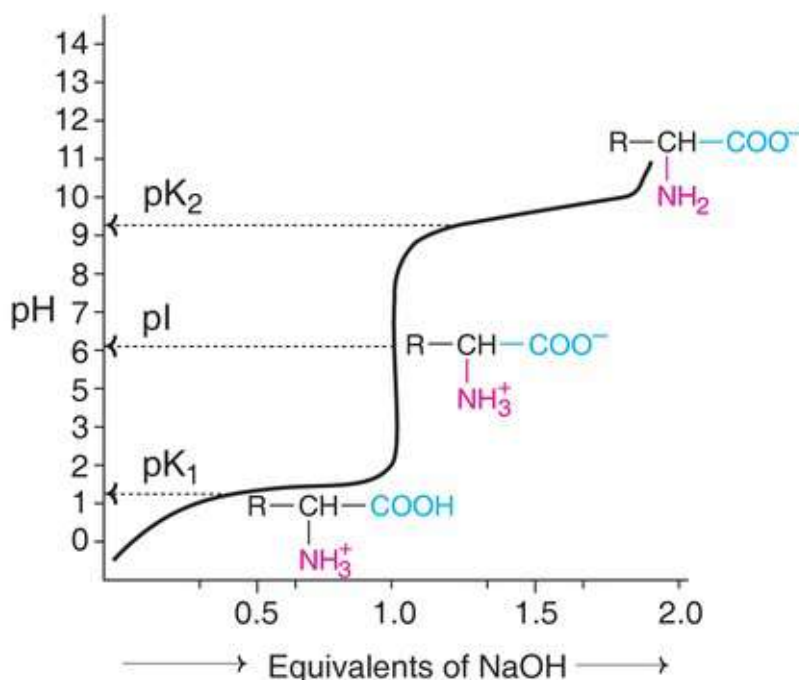
FIG. 4.3 Titration curve of an amino acid-leucine ( R = (CH_3)_2CH-CH_2 —; pK_1 = Dissociation constant for COOH; pI = Isoelectric pH; pK_2 = Dissociation constant for NH_3^+ ).
