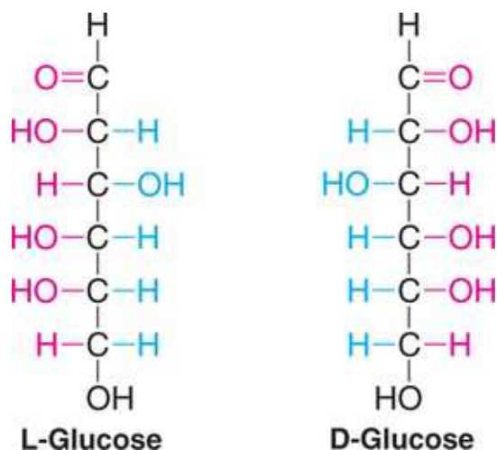
FIG. 2.5 Enantiomers (mirror images) of glucose.
