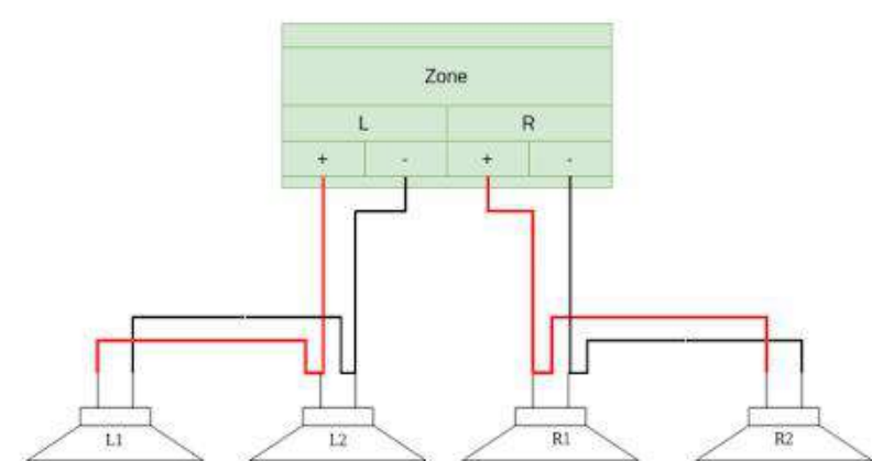
Doubling Up a Zone – 4 speakers into one zone (must be 8ohm speakers and can only be done on 2 zones per Juke)
