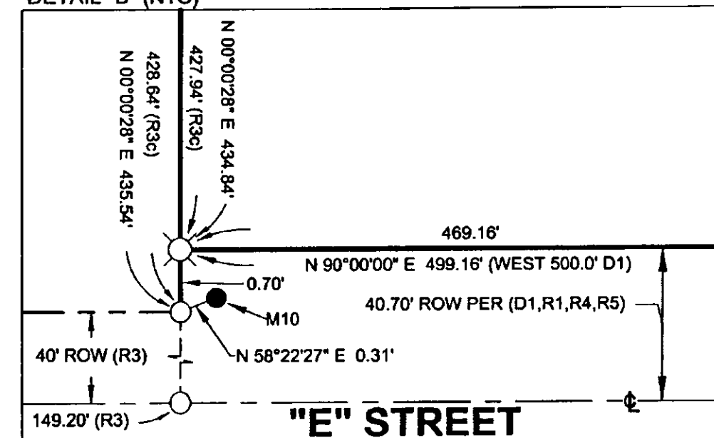
DETAIL "B" (NTS)
