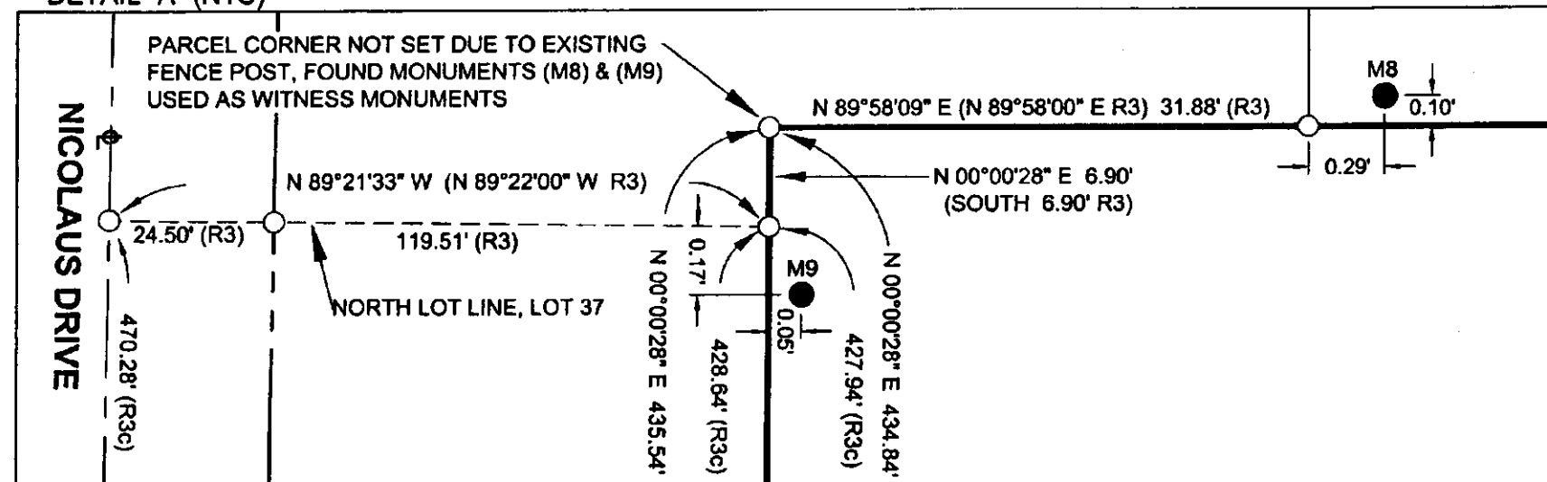
DETAIL "A" (NTS)
