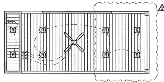
2 CEILING & ELECTRICAL PLAN SCALE: 1/4" = 1'-0"
