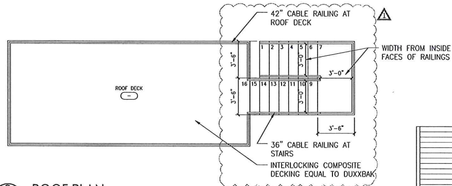
3 ROOF PLAN SCALE: 1/4" = 1'-0"
