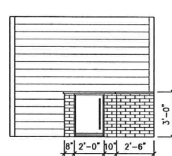
4 INTERIOR ELEVATION SCALE: 1/4" = 1'-0"
