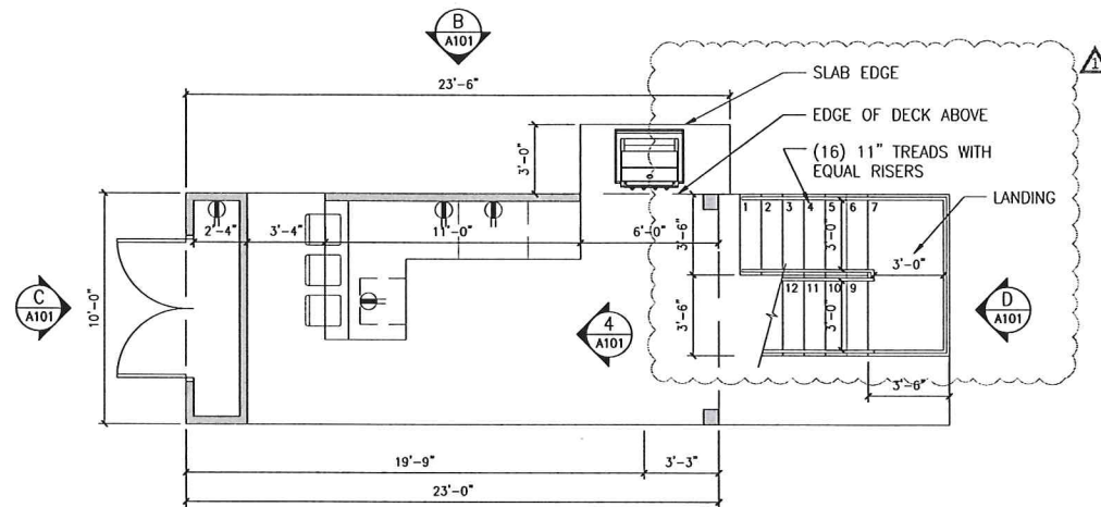
1 FLOOR PLAN SCALE: 1/4" = 1'-0"
