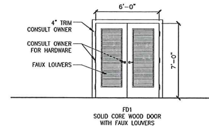
5 DOOR DETAIL SCALE: 1/4" = 1'-0"
