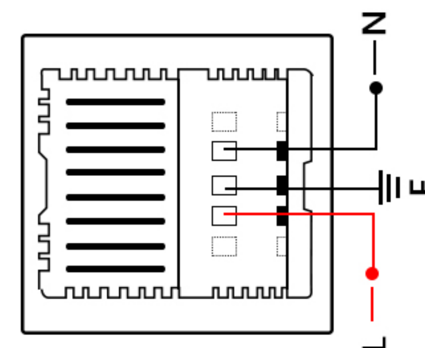
Wiring Diagram
