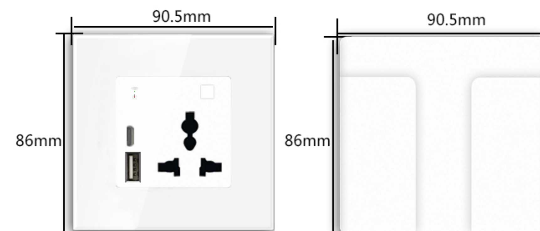
Size Diagram
