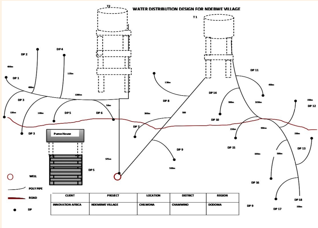
Ndebwe Water Distribution System Design
