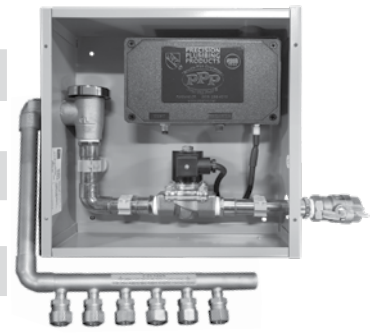
(SURFACE MOUNT)
