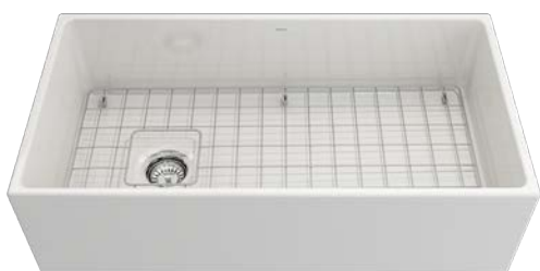
1354-XXX-0120 Apron-Front Single Bowl 36" x 19" x 10" 99.65 lbs min. 39" wide base cabinet for apron sinks required
