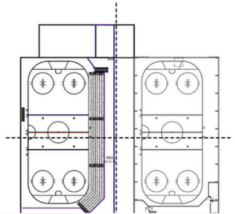
LEVEL 1-OCCUPANCY 117' x 117'
